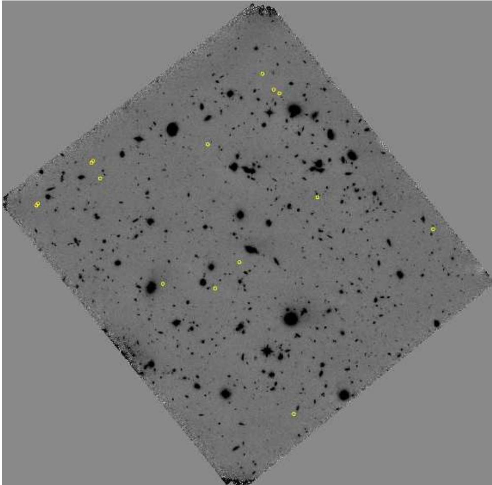
Figure 4. The positions of the 15 galaxies in our sample with primary photometric redshift solutions at z > 7 overplotted on the new WFC3/IR H_{160} -band image of the HUDF (North is up, and East is to the left). The 4 most distant galaxies in the sample (at z > 7.8 ) are confined to the groups at the north and north-east of the image.
