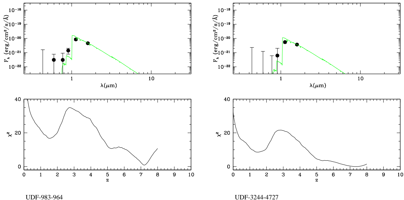
Figure 1. The results of our SED fitting to the optical (ACS) and near-infrared (NICMOS F110W & F160W) photometry for the two most plausible galaxy candidates at z > 7 discovered within the HUDF prior to the new WFC3/IR imaging campaign. The upper panels show the best-fitting SED while the lower panels show the dependence of \chi^2 on redshift (marginalised over all other fitted parameters).
