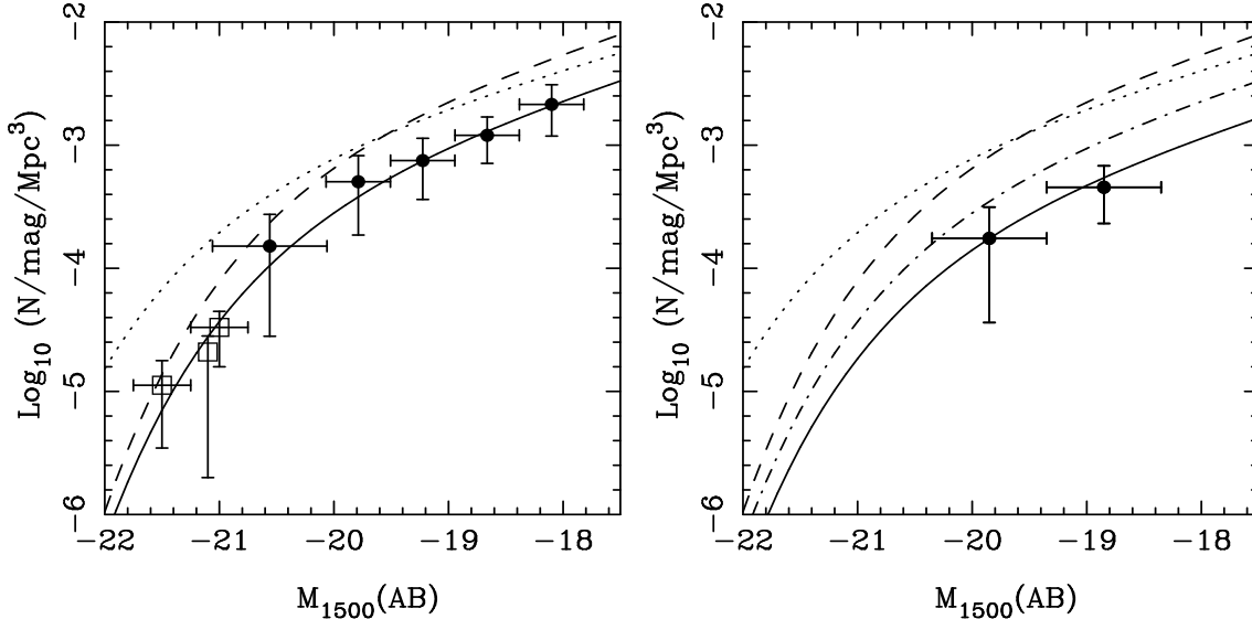
Figure 5. Our new determinations of the ultraviolet (UV) galaxy luminosity function at z \simeq 7 and z \simeq 8 . The left-hand panel shows our V/V_{\max} estimate of the redshift z = 7 luminosity function. The absolute UV magnitudes have been calculated at a rest-frame wavelength of 1500\text{\AA} . The filled circles are the data-points from this study, where the horizontal error bars indicate the width of the magnitude bins adopted (either \Delta m = 0.5 or \Delta m = 1.0 depending on signal-to-noise) and the vertical error bars indicate the uncertainty due to simple Poisson statistics. The open squares are taken from the ground-based study of the Subaru Deep Field and GOODS-North field by Ouchi et al. (2009). The dotted and dashed curves are the Schechter function fits to the z = 5 and z = 6 luminosity function from McLure et al. (2009). The solid line is our best-fitting Schechter function to the z = 7 luminosity function. The right-hand panel shows our corresponding estimate of the luminosity function at redshift z = 8 . In this panel the dashed and dot-dashed curves are the z = 6 and z = 7 Schechter function fits from McLure et al. (2009) and this work respectively. The solid line is the best-fitting z = 7 Schechter function with \phi^* reduced by a factor of two (see text for a discussion).
