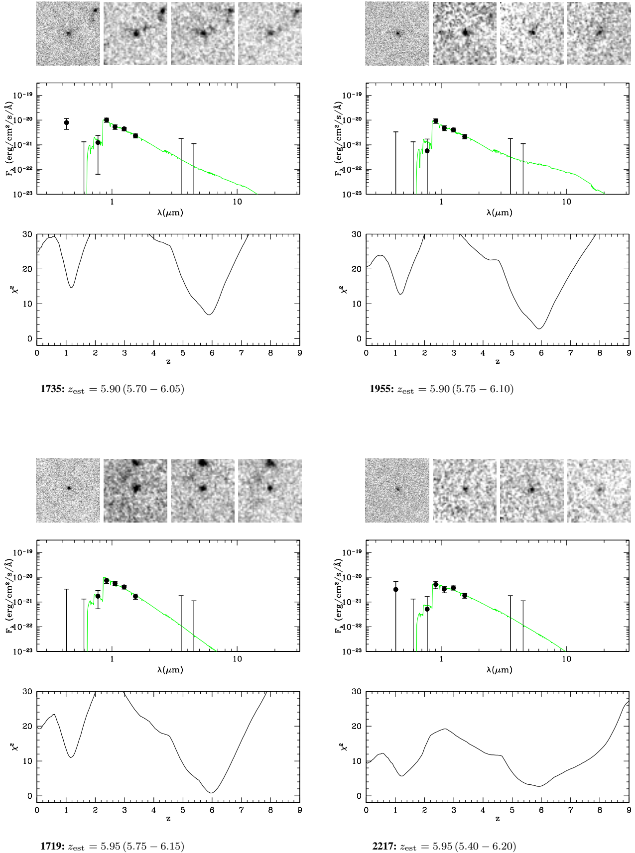
Figure A1. 3 \times 3 arcsec z_{850} , Y_{105} , J_{125} , H_{160} (left to right) greyscale ( -2\sigma – +6\sigma ) postage-stamp images are shown for each galaxy candidate above a plot which shows the galaxy SED which best fits the HST ACS optical, WFC3/IR near-infrared and Spitzer 3.6\mu\text{m} and 4.5\mu\text{m} photometric limits. The lower panel for each object shows how \chi^2 varies with redshift, marginalised over galaxy age, star-formation history, and dust reddening. The ID number of each source, and its estimated redshift (with 1\sigma error range) are given under each plot.
