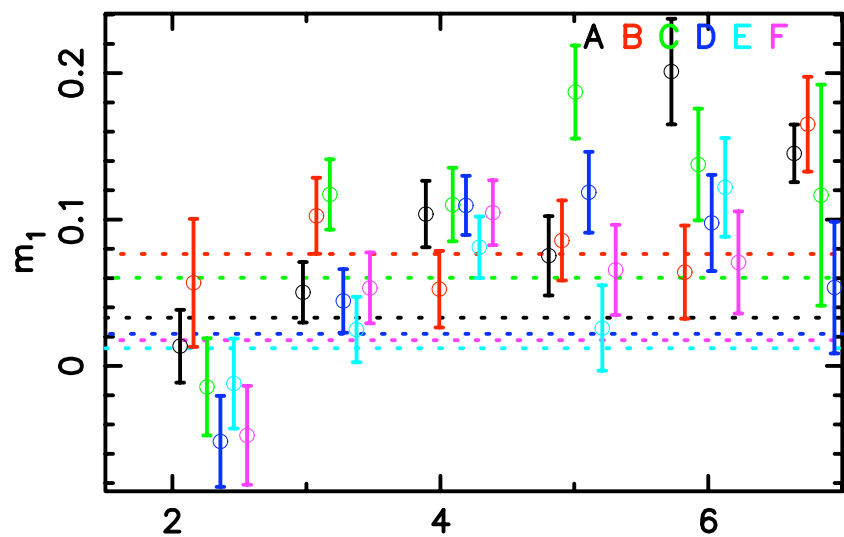
Shapelet Size
