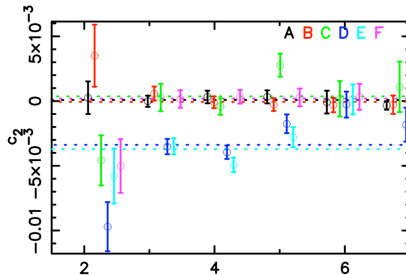
Shapelet Size
