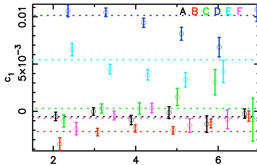
Shapelet Size
