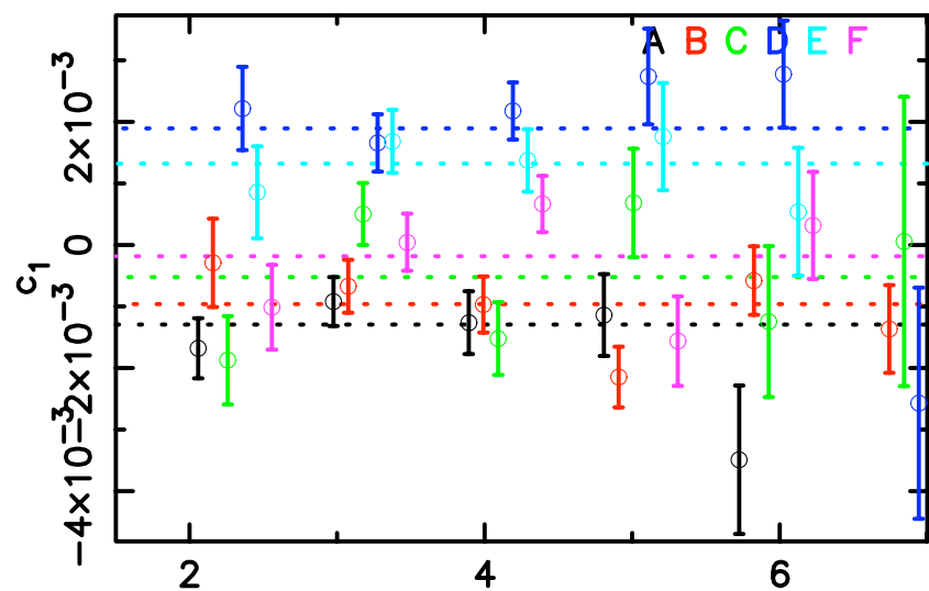
Shapelet Size
