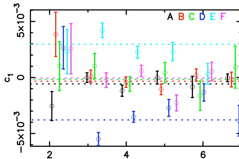
Shapelet Size
