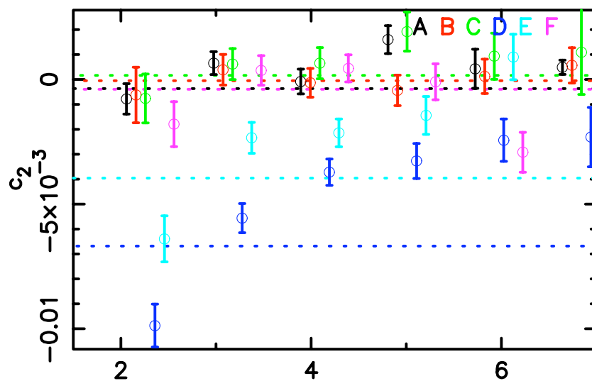
Shapelet Size
