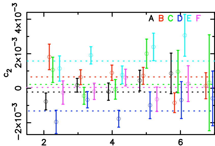
Shapelet Size
