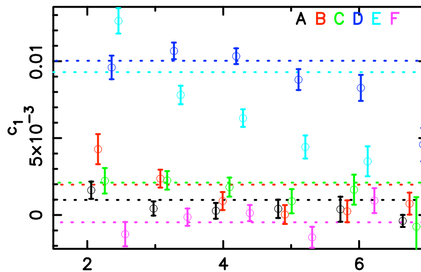
Shapelet Size
