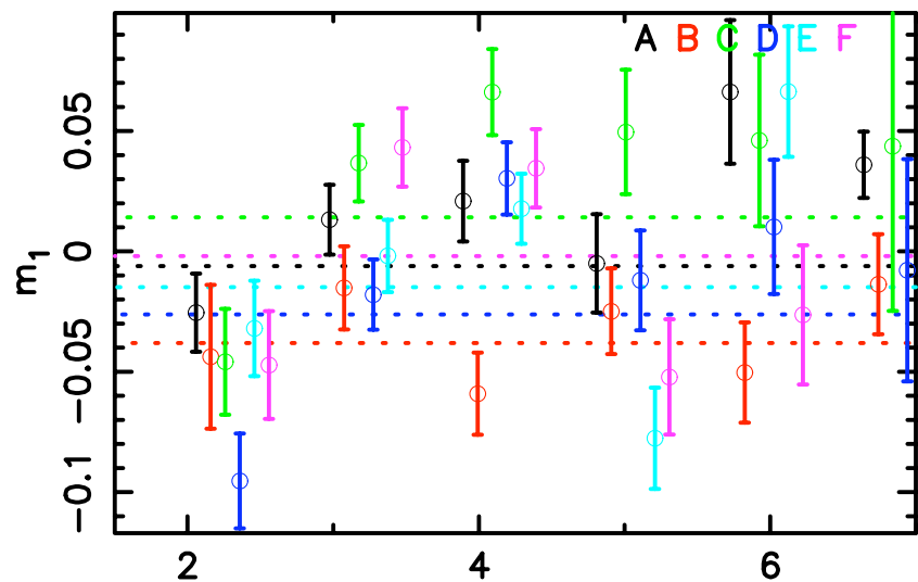
Shapelet Size
