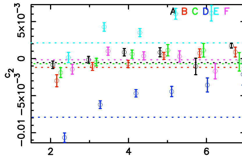
Shapelet Size
