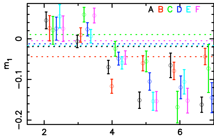
Shapelet Size
