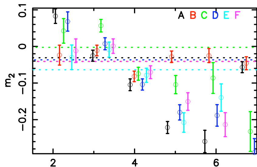
Shapelet Size
