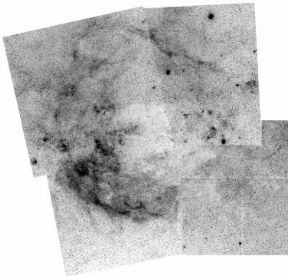
Figure 1 —The Coalsack Loop. Composite of four H \alpha images centred on the ESO/SERC Sky Survey fields 95, 96, 131 and 132. Note the presence of the Southern Cross in the upper-right (north-west) portion of the image.
