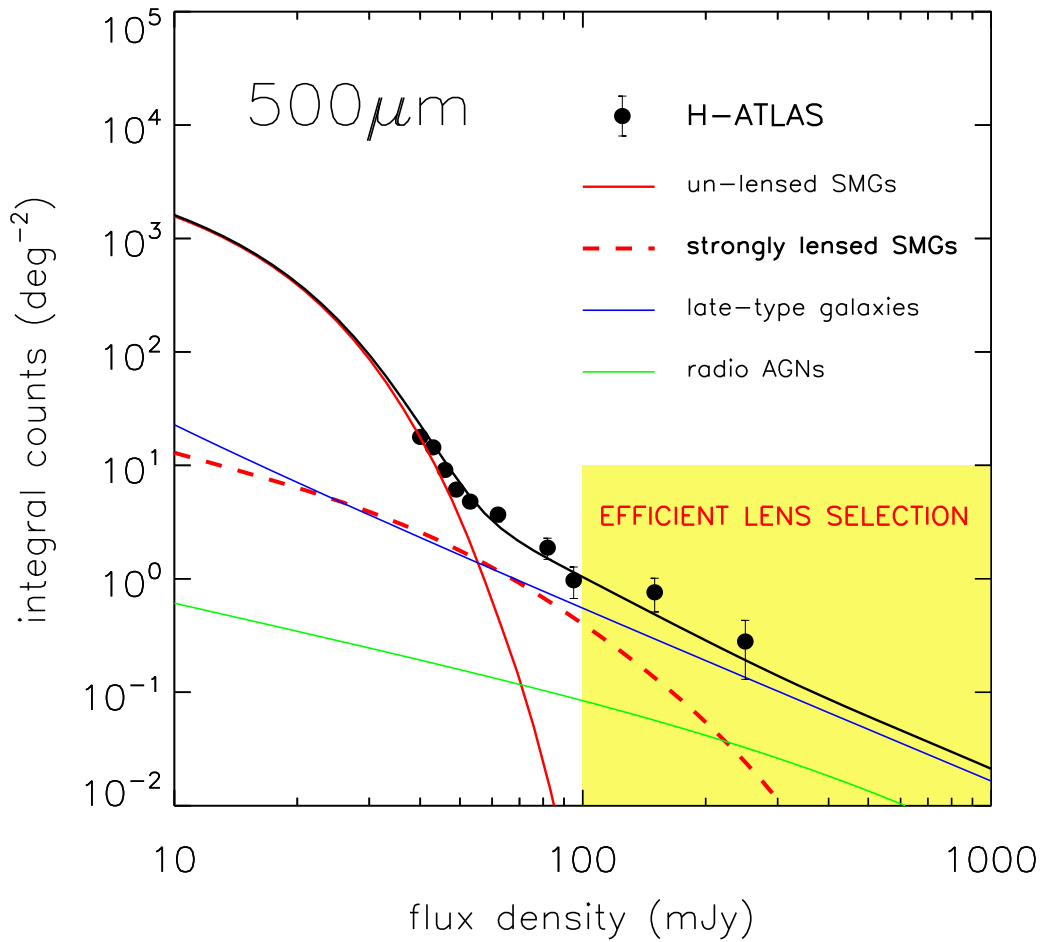
Figure 1: Selection of gravitational lenses at sub-mm wavelengths. The 500 \mu\text{m} source counts consist of three different populations (14): high-redshift dust-obscured starforming galaxies (SMGs); low redshift z < 0.1 late type (starburst plus normal spiral) galaxies; and radio sources powered by active galactic nuclei. Strongly lensed SMGs dominate over unlensed SMGs at very bright fluxes where the count of un-lensed SMGs falls off dramatically (yellow shaded region). The data points are from H-ATLAS (33).
