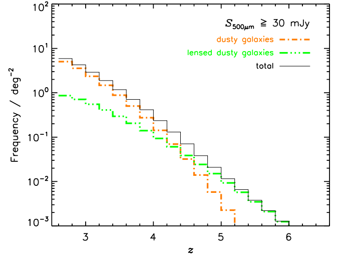
Figure 10. Redshift distribution of S_{500} > 30\text{-mJy} sources from the physical model of Cai et al. (2013) which provides a good fit to a broad variety of data, including the IR luminosity functions determined observationally by Grupponi et al. (2013) at several redshifts up to z \sim 4 (see also Figure 1 of Bonato et al. 2014). The dot-dashed green histogram and the dot-dashed orange histogram show the contributions of strongly lensed (magnification, \mu \geq 2 ) and unlensed galaxies, respectively, while the black histogram shows the total. The distribution of lensed galaxies was computed using the SISSA model (Lapi et al. 2012). Although strongly lensed galaxies are a minor fraction of all galaxies with S_{500} > 30\text{mJy} , they become common at z > 4 due to the combined effect of the increase with redshift of the optical depth to lensing and the magnification bias. This will be addressed in a forthcoming paper, in which we present high-resolution ALMA imaging (Oteo et al. 2016b).
