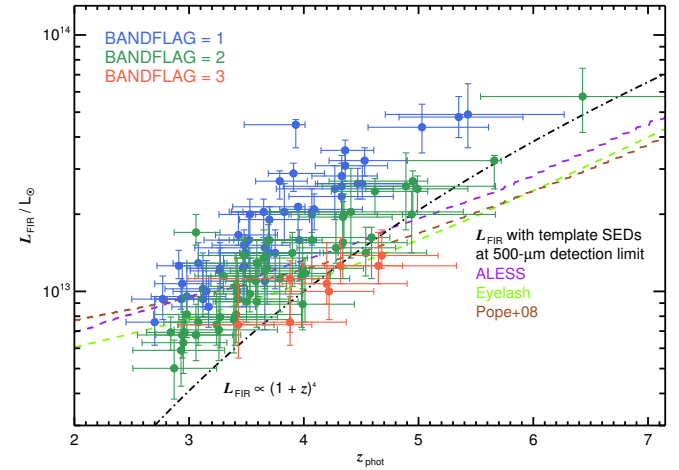
Figure 11. L_{\text{IR}} as a function of z_{\text{phot}} for our sample, color-coded by BANDFLAG, with the S_{500} > 30\text{-mJy} detection limits shown for our three best SED templates, and luminosity evolution of the form \propto (1+z)^4 illustrated. We see that the BANDFLAG = 1, 2 and 3 galaxies lie in distinct regions, as one might expect. The least luminous galaxies at any redshift are those detected only in the 500- \mu\text{m} filter, since in the SPIRE maps with the lowest spatial resolution they suffer considerably more flux boosting and blending. The growing gap between the galaxies and the expected detection limits at z > 5 is potentially interesting.
