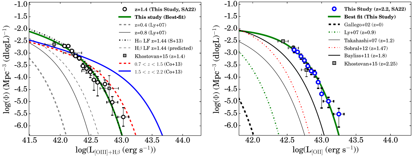
Figure 12. Left: observed [\text{O III}] + \text{H}\beta LF at z \sim 1.4 from our SA22 survey and comparison with other studies/surveys (including the LF from UDS+COSMOS derived by Khostovan et al. 2015). Our results clearly show that the [\text{O III}] + \text{H}\beta LF is evolving very strongly with redshift, mostly due to a strong increase in L^* , similarly to the behaviour of the \text{H}\alpha LF. Our best fit is very similar to the observed \text{H}\alpha LF at the same redshift (also shown), and, at the faint end, reveals a higher number of [\text{O III}] + \text{H}\beta emitters than in Colbert et al. (2013) – these are likely explained by a combination of \text{H}\beta emitters (we also show our predicted \text{H}\beta LF based on the \text{H}\alpha LF from Sobral et al. 2013a), but also due to the prevalence of the [\text{O III}] 4959 line (see Section 4.2). The deviations from a Schechter function are likely explained by the mix of different lines contributing to the final LF, as the observed LF is likely a combination of three different functions (for the three different emission lines). For higher luminosities, our data is in good agreement with the results from Colbert et al. (2013) and our slightly lower number densities are likely a result of accounting for the contribution of both [\text{O III}] 4959 and \text{H}\beta for the final value probed. Most importantly, we compare our results with Khostovan et al. (2015), who present the [\text{O III}] + \text{H}\beta LF from HiZELS in COSMOS+UDS, and find a very good agreement. Right: [\text{O II}] LF at z = 2.2 from our SA22 survey and comparison with other lower redshift surveys such as Gallego et al. (2002), Takahashi et al. (2007) and Bayliss et al. (2011). Similarly to the evolution of the \text{H}\alpha and [\text{O III}] + \text{H}\beta LFs, the [\text{O II}] LF shows a strong L^* evolution. Such increase in L^* with increasing redshift is even stronger by a few times than what is seen for other lines. On the other hand, there is little to no evidence of evolution in \phi^* . We also compare our results from SA22 with those from UDS and COSMOS (HiZELS) presented by Khostovan et al. (2015) and find a very good agreement, at both the bright and faint ends.
