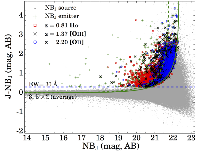
Figure 2. Colour–magnitude diagram for our \text{NB}_J detected sources. The dotted horizontal line is for an observed EW of 30 \text{ \AA} , which corresponds to J - \text{NB}_J = 0.3 . The 3\sigma and 5\sigma selection curves are shown for the average depth of the survey for reference (but note that some small variations exist across the survey). Candidate line emitters that passed the EW, \Sigma and visual filtering (to exclude spurious sources or artefacts) are shown in colour, while all other non-excess sources are shown in grey. Emitters classed as \text{H}\alpha ( z = 0.81 ), [\text{O III}] ( + \text{H}\beta ) at z = 1.37 and [\text{O II}] at z = 2.2 , or unclassified, are plotted in different colours as indicated by the key. Note that, as expected, higher redshift emitters are always preferentially found at fainter and fainter magnitudes. Thus, for example, a survey a magnitude shallower would recover little to no [\text{O II}] emitters at z = 2.2 .
