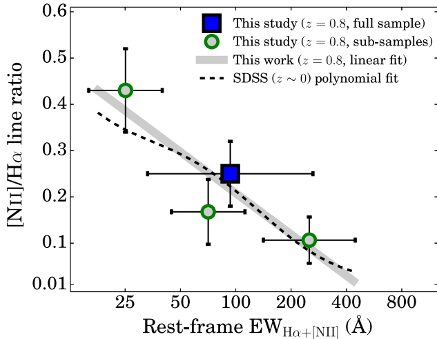
Figure 9. The observed anticorrelation between the [\text{N II}]/\text{H}\alpha line ratio and the rest-frame \text{EW}(\text{H}\alpha + [\text{N II}]) at z = 0.81 in this study and a comparison with the polynomial fit to SDSS at low redshift. Given the range of EWs and line ratios probed, we find that while the SDSS fit is a good fit to the data at z = 0.81 , a linear fit does equally well, and is a much simpler way to robustly estimate [\text{N II}]/\text{H}\alpha . The relation is f([\text{N II}]/\text{H}\alpha) = -0.296 \times \log_{10}(\text{EW}_{\text{H}\alpha + [\text{N II}]}) + 0.8 . We show three bins which split the sample in three relatively evenly in parameter space and that do not overlap, together with the stack for the full sample, and three other stacks which split the sample in terms of number of \text{H}\alpha emitters.
