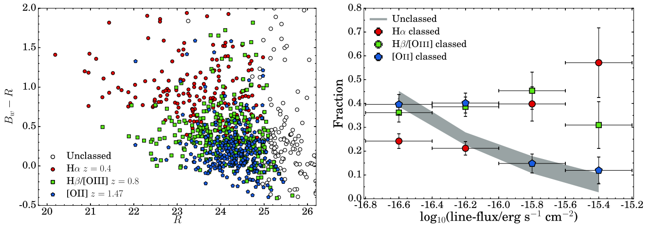
Figure 2. Left: B_w - R versus R colour–magnitude diagram of line-emitters in NB921. This plot illustrates that the line-emitters that are not detected in enough broad-bands (such as I , z or H ) in order to be classified, are typically faint ( R > 25.5 , note that these are low S/N detections) and lie most closely to the colour–magnitude parameter space probed filled with [O II] emitters. Right: the fraction of sources classed as H\alpha , H\beta/[O III] and [O II] amongst the classed NB921 line-emitters in bins of line-flux. The grey-shaded area shows the fraction of sources that is unclassified and its Poissonian uncertainty. All emitters at higher line-fluxes are classed. These fractions are used to correct for identification incompleteness (Section 5.1.3).
