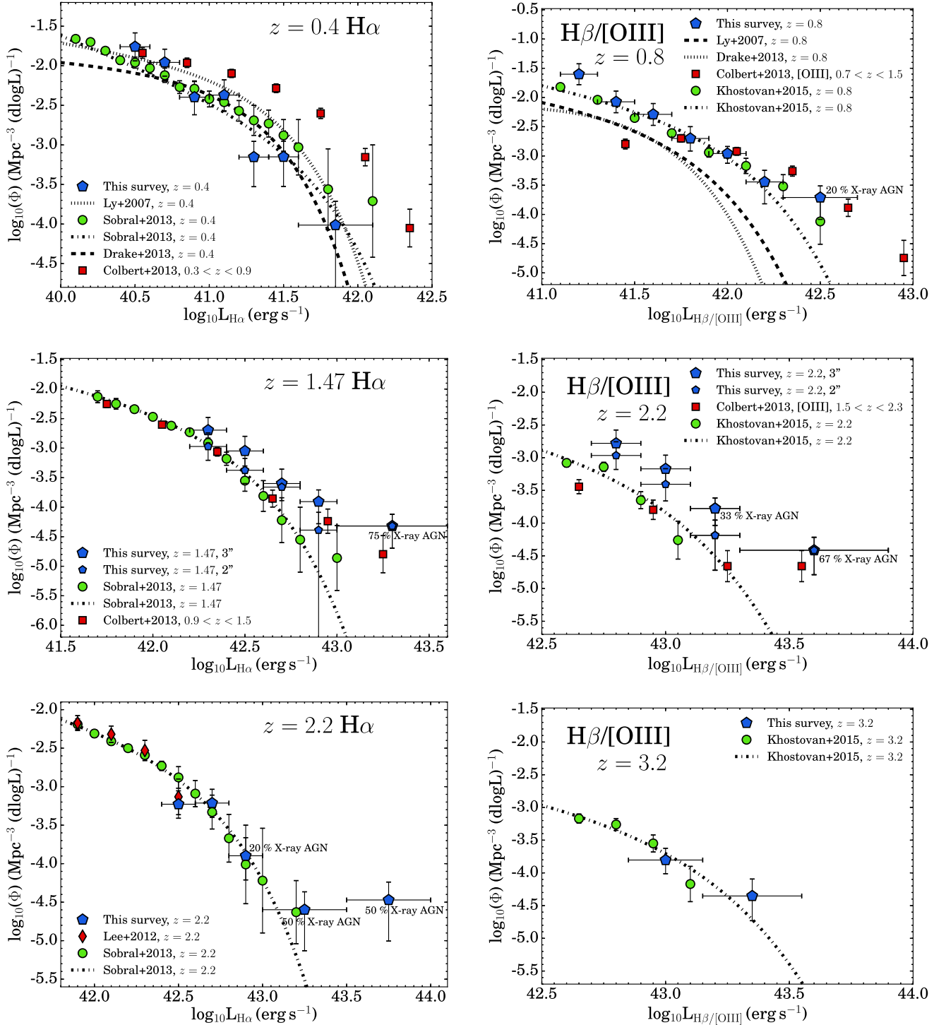
Figure 4. Left column: measured H\alpha LFs at z = 0.4 , 1.47 , 2.2 . H\alpha luminosities are corrected for the [NII] contribution using a relation with H\alpha +[NII] EW (Sobral et al. 2012), but are not corrected for dust. At z = 0.4 , the LF is compared to the narrow-band survey from Ly et al. (2007) in the Subaru Deep Field (SDF) field and Drake et al. (2013) in the UDS field and with the survey from Lee et al. (2012) at z = 2.2 . At all redshifts, the number densities are compared to the HiZELS survey results in the UDS+COSMOS fields from Sobral et al. (2013). We also compare the LFs with those measured in a blind grism survey by Colbert et al. (2013). Overall, there is reasonable agreement. The luminosity-offset at z = 1.47 may be explained by aperture effects (see Section 5.2.2). The brightest bin at z = 2.2 is due to the presence of (spectroscopically confirmed) AGN. Right column: measured H\beta/[OIII] LFs at z = 0.8 , 2.2 , 3.2 , compared to Ly et al. (2007) and Drake et al. (2013) at z = 0.8 and to Khostovan et al. (2015) and Colbert et al. (2013) at higher redshift. There is a luminosity-offset at z = 2.2 that is partially due to a larger aperture measuring a higher luminosity by \approx 0.14 dex (this is the same filter as the H\alpha LF at z = 1.47 ). The brightest bin at z = 2.2 contains the same AGN as in the brightest bin of the H\alpha LF at z = 2.2 .
