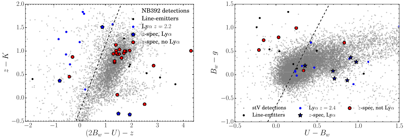
Figure B1. Colour selection criteria used to select LAEs at z = 2.2 and z = 2.4 . These are based on the BzK criterion from Daddi et al. (2004). The B_w band magnitude is adjusted for the contribution to flux in the U band. We highlight the sources with spectroscopic redshifts in larger symbols.
