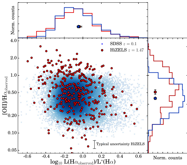
Figure 7. Observed [\text{O II}]/\text{H}\alpha ratio as a function of observed \text{H}\alpha luminosity, normalized by the typical luminosity ( L^* ) at either z = 1.47 ( L^* = 10^{42.16} \text{ erg s}^{-1} ; Sobral et al. 2013) or z = 0.1 ( L^* = 10^{41.4} \text{ erg s}^{-1} ; Ly et al. 2007). The blue points (coloured by density) show the ratios observed in SDSS at z = 0.1 , while the red points show the HiZELS measurements at z = 1.47 . The distribution of L/L^* is similar at both redshifts, while the median observed [\text{O II}]/\text{H}\alpha increases from 0.40 \pm 0.01 in the local Universe to 0.52 \pm 0.05 at z = 1.5 . A KS test confirms that this increase is statistically significant. This increase could be due to evolution of the dust attenuation, or an effect from fibre-measurements in SDSS.
