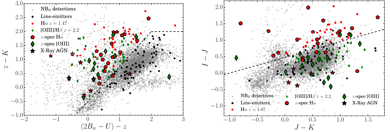
Figure B4. Colour criteria used to classify line-emitters identified with the NB H filter. The modified B_w zK criterion is used to distinguish z > 1 line-emitters from z < 1 line-emitters. We then distinguish between z = 1.47 and z = 2.2 based on the positions of Balmer breaks. At z \approx 1.5 , the Balmer break lies around an observed 1000 nm, hence between I - J (note that we use I rather than z because I is deeper and broader, see Table 1). At z \approx 2.2 , the Balmer break lies between the J and K bands. Note that several X-ray-detected H \alpha emitters at z = 1.47 mimic the colours of z = 2.2 [O III]/H \beta emitters. These sources typically have high line-fluxes and their spectroscopic follow-up completeness is high. [O II] emitters at z = 3.3 are selected based on the position of their Lyman-break, similar to LAEs at z = 3.1 in Fig. B2.
