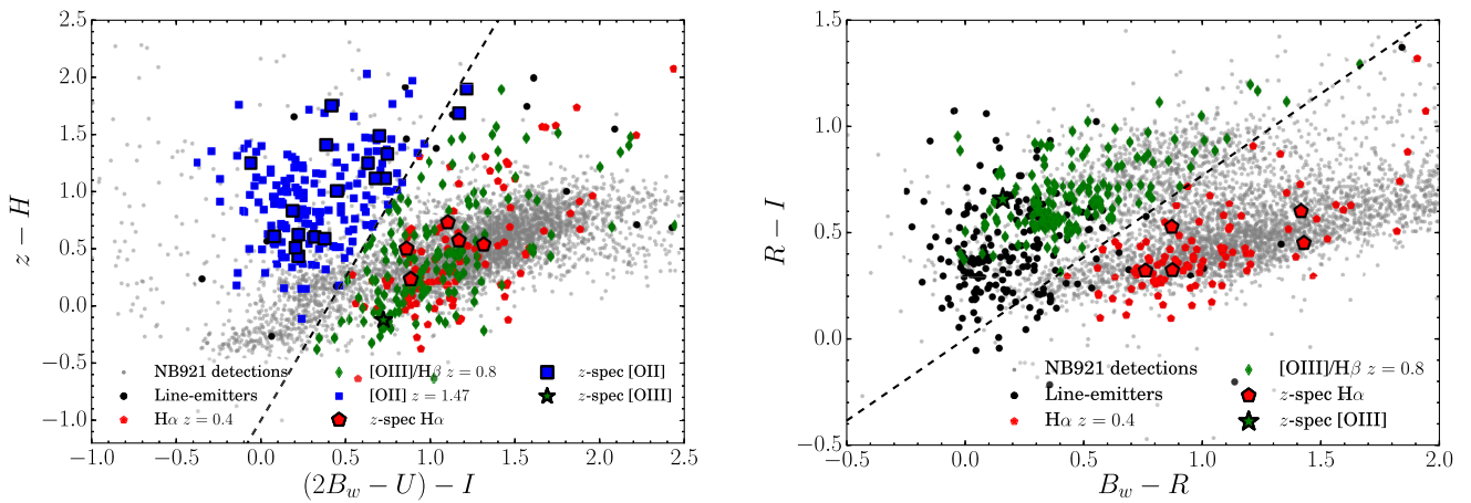
Figure B3. Colour selection criteria used to distinguish H\alpha , [O\text{ III}]/H\beta and [O\text{ II}] emitters amongst the line-emitters identified with NB921. The criterion in the left-hand panel identifies Balmer breaks at specific redshift intervals. Because this criterion cannot distinguish between z = 0.4 and z = 0.8 , we use the additional B_w R I colours to distinguish between a Balmer break between B_w and R (around 600 nm, or z \approx 0.5 ) and between R and I (around 700 nm, or z \approx 0.75 ).
