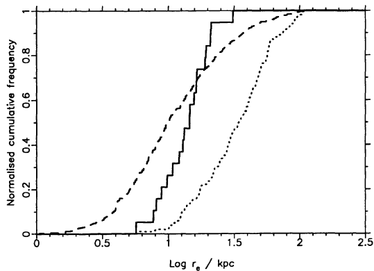
Figure 10. Normalized cumulative frequency distributions of r_e for the three different populations of galaxies: solid line – the high-redshift 3CR galaxies; dotted line – low-redshift brightest cluster galaxies; dashed line – low-redshift elliptical galaxies (excluding brightest cluster galaxies). The 3CR galaxies have a much smaller spread in r_e than the low-redshift elliptical galaxies.
