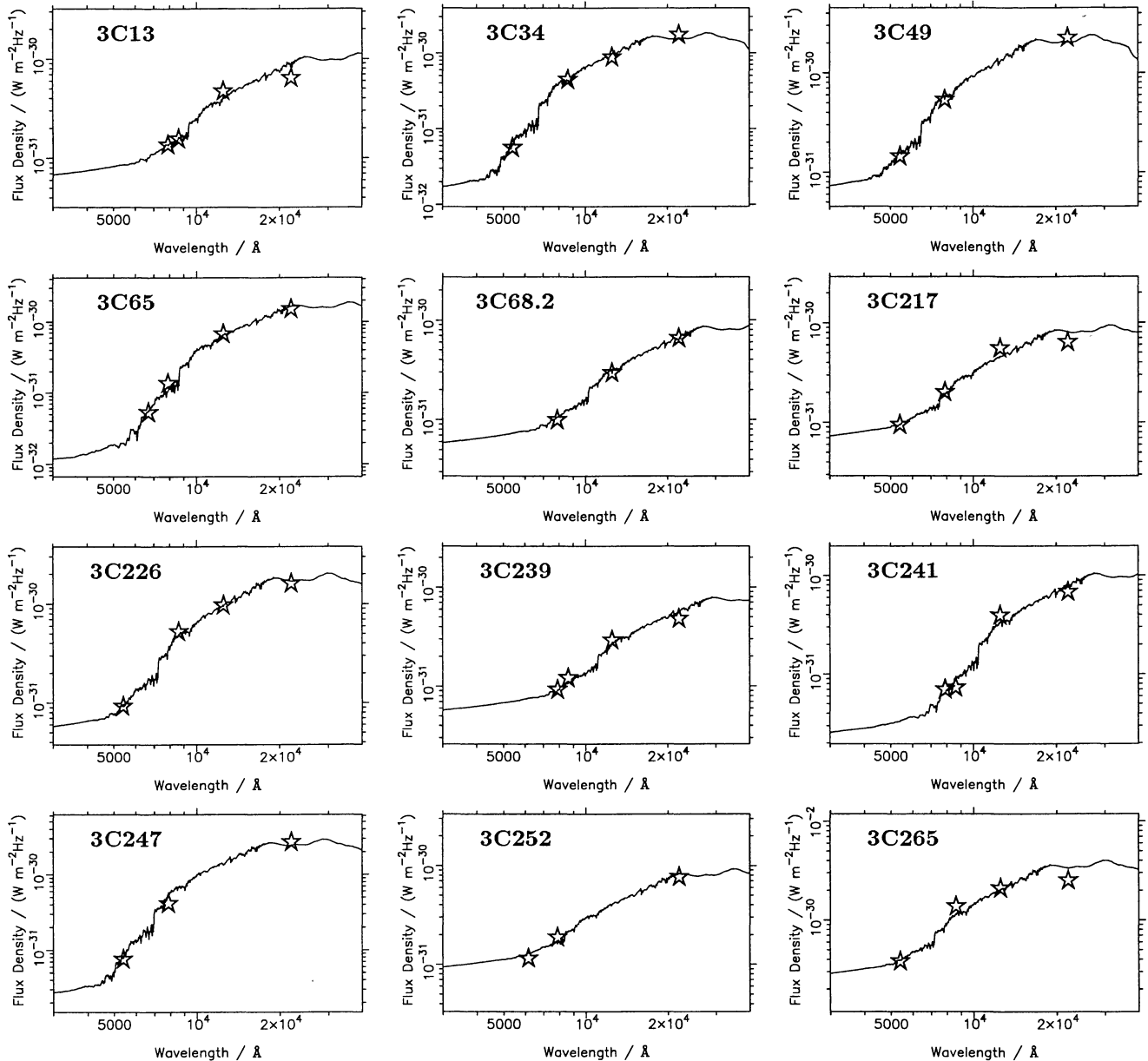
Figure 1. SED fits to the broad-band flux densities of the 3CR galaxies using an old stellar population and an aligned component (see text and Table 2 for details).
