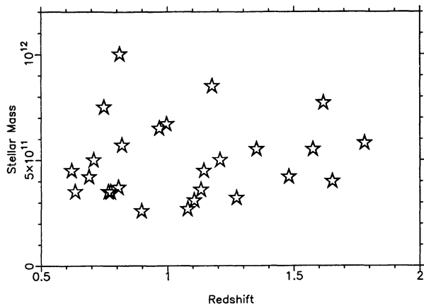
Figure 13. A plot of the stellar mass derived by a fit to the broad-band photometry of Section 3 against redshift for 26 3CR galaxies.
