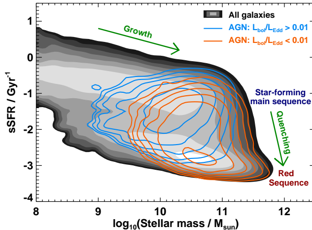
Fig. 2.— The distribution of galaxies in the SDSS main galaxy sample on the plane of stellar mass vs. specific star formation rate ( sSFR = SFR/M_* ). The greyscale indicates the volume-weighted distribution of all galaxies, with each lighter color band indicating a factor of two increase. Galaxies predominantly fall within two regions: a ‘main sequence’ of star-forming galaxies, and a red sequence of ‘quenched’ galaxies. The blue and red contours show the volume-weighted distributions of high ( >1\% ; mostly radiative-mode) and low ( <1\% ; mostly jet-mode) Eddington-fraction AGN, with contours spaced by a factor of two.
