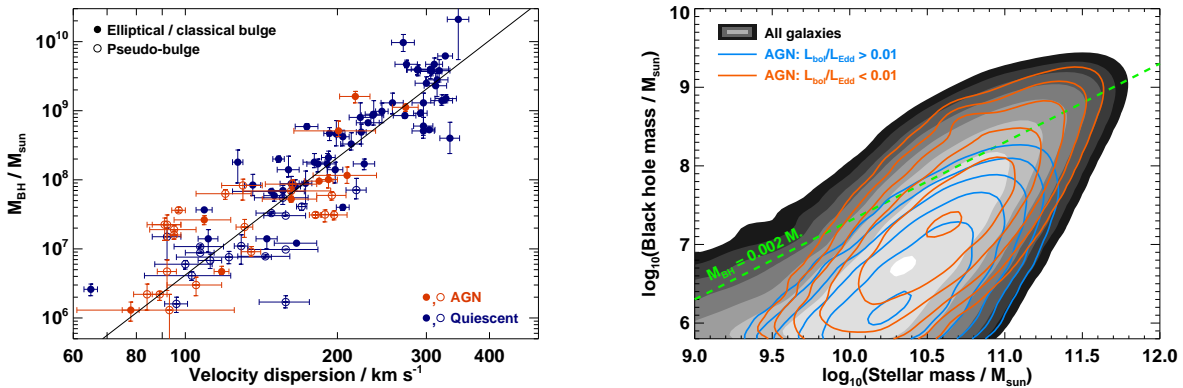
Fig. 9.— Left: The M_{\text{BH}}-\sigma relation of local galaxies with direct black hole mass measurements (data from Woo et al. 2013 and references therein). Both AGN (the color-coding includes both radiative-mode and jet-mode AGN) and quiescent galaxies are consistent with the McConnell & Ma (2013) relation, shown by the solid line. Right: The distribution of galaxies in the SDSS main galaxy sample on the stellar mass vs. black hole mass plane, using black hole masses derived from the M_{\text{BH}}-\sigma relation. The greyscale indicates the volume-weighted distribution of all galaxies, with each lighter color band indicating a factor of two increase. It is clear that the black hole mass is not a fixed fraction of the total stellar mass. This is also true for AGN: the blue and red contours show the volume-weighted distributions of high ( >1\% ; mostly radiative-mode) and low ( <1\% ; mostly jet-mode) Eddington-fraction AGN, with contours spaced by a factor of two.
