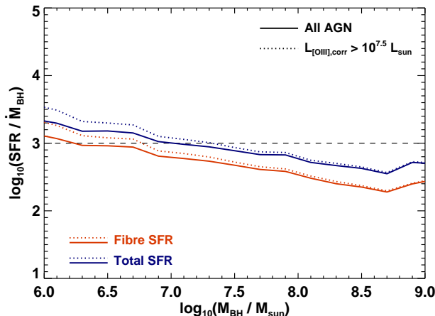
Fig. 23.— Ratio of the total star formation rate per unit volume in galaxies to the total accretion rate per unit volume onto black holes as traced by Type 2 AGNs, plotted as a function of the black hole mass. The sample studied consists of all galaxies from the SDSS main galaxy sample with stellar surface mass density above the characteristic value \mu_* = 10^{8.5} M_\odot \text{ kpc}^{-2} . Red lines show the result if the SFR is calculated within the fiber aperture for each galaxy and the blue lines show the result using estimates of the total SFR. Dotted lines show results restricted to the AGNs with (reddening corrected and star-formation corrected) L_{[\text{OIII}]} > 10^{7.5} L_\odot . The horizontal dashed line shows the fiducial value of stellar to black hole mass in bulges and elliptical galaxies. Adapted from Heckman et al. (2004).
