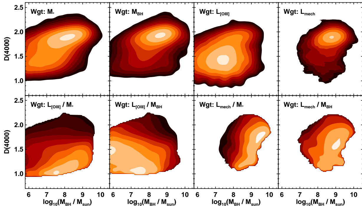
Fig. 15.— As Fig. 14, but now showing the distributions in the black hole mass vs. 4000Å break strength plane.
