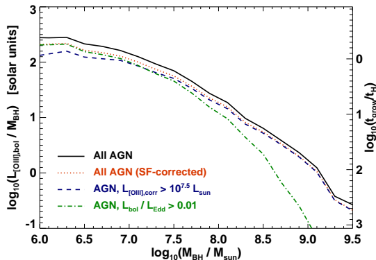
Fig. 10.— Logarithm of the ratio of the total bolometric radiated luminosity (as calculated from the [OIII] emission line; see Section 2.3.1) per unit volume due to emission-line AGN of a given black hole mass to the total mass per unit volume in black holes at that black hole mass (both in solar units) in the contemporary universe. The right axis shows the corresponding growth time (mass-doubling time) for the population of black holes in units of the Hubble time. The solid black line shows the result obtained by integrating over all AGNs in the sample. The dotted red line shows the effect of correcting the [OIII] luminosities for the contribution from star formation in composite galaxies. The dashed blue line shows the result obtained if only AGN with (reddening-corrected and star-formation corrected) [OIII] luminosities above 10^{7.5} L_{\odot} are included. The dash-dot green line includes only AGN with bolometric luminosities above 1% of the Eddington rate (this cut effectively reduces the sample to only radiative-mode AGN). Adapted from Heckman et al. (2004).
