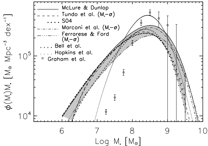
Fig. 13.— A collection of estimates of the distribution of mass across the local black hole population (ie., the local black hole mass function scaled by black hole mass) taken from Shankar et al. (2009). The shaded grey area represents the range of estimates based on local scaling relations of M_{\text{BH}} with \sigma , M_{\text{Bulge}} , and L_{\text{Bulge}} . See Shankar et al. (2009) for details.
