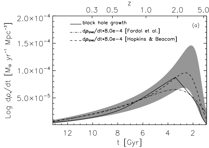
Fig. 1.— The cosmic history of black hole growth and stellar mass growth. The average black hole accretion rate is compared to the SFR as a function of redshift, where the latter is given by Hopkins & Beacom (2006) and Fardal et al. (2007), scaled by the factor 0.8 \times 10^{-3} . The shaded grey area shows the 3\sigma uncertainty region from Hopkins & Beacom (2006). Figure from Shankar et al. (2009).
