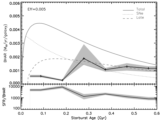
Fig. 18.— Top Panel: the mean black hole accretion rate (BHAR) averaged over all galaxies in a sample of starburst and post-starburst galaxies (black line). The grey-shaded area shows the typical 10th and 90th percentile range on the total BHAR estimated from bootstrap resampling of the data. The model prediction for the average gas mass-loss rate from the stars formed during the starburst (solid grey line) assumes an accretion efficiency onto the black hole of 0.5 per cent of the ejecta from intermediate and low-mass stars between the age of 250 and 600 Myr. Stars return mass to the ISM through supernova explosions and fast winds from massive stars (dotted line) and planetary nebula ejections and stellar winds from lower mass stars (dashed line). Bottom panel: the ratio of SFR (from H\alpha ) to BHAR, with mean value and errors calculated as for the top panel. The BHAR lags the SFR and becomes significant only after several hundred Myr. Figure from Wild et al. (2010).
