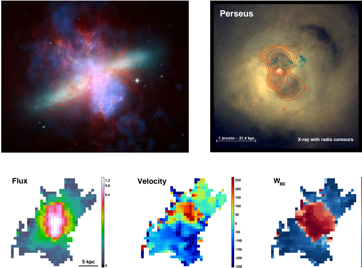
Fig. 21.— Illustrative examples of feedback effects at work. The upper-left panel shows the ‘Great Observatories’ composite image of the starburst-driven galactic wind in M82: visible light is shown in yellow-green, infrared emission in red, H \alpha emission in orange and X-ray emission in blue (Credit: NASA/JPL-Caltech/STScI/CXC/UofA/). The upper-right panel shows jet-mode feedback in the Perseus cluster (data from Fabian et al. 2006). The color-scaling shows the X-ray emission, colored such that hard X-rays are in blue and soft X-rays in red. The contours indicate the radio emission, which can be seen to have evacuated cavities in the X-ray gas. The three lower panels illustrate AGN-driven feedback from a high luminosity radiative-mode AGN (reproduced from Liu et al. 2013b). They show, respectively, the surface brightness (in units of 10^{-14}\text{ergs}^{-1}\text{cm}^{-2}\text{arcsec}^{-2} ), relative velocity (in \text{kms}^{-1} ), and velocity width ( W_{80} is the velocity width in \text{kms}^{-1} containing 80% of the emitted line flux) of the [OIII] emission line in the Type 2 QSO SDSS J0319-0019.
