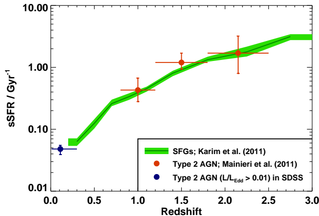
Fig. 22.— The specific star formation rate ( sSFR = SFR/M_* ) of radiative-mode AGN hosts compared to normal star-forming galaxies, as a function of redshift. The green shaded region shows the evolution of the sSFR of galaxies along the star-forming main sequence derived by Karim et al. (2011). The red points show the sSFR of the host galaxies of X-ray selected Type 2 AGN from the XMM-COSMOS field derived by Mainieri et al. (2011). The blue point indicates the average sSFR of emission-line selected Type-2 AGN with L/L_{Edd} > 0.01 (ie. broadly radiative-mode) from the SDSS. At all redshifts, the sSFR of radiative-mode AGN hosts are consistent with those of galaxies on the star-forming main sequence.
