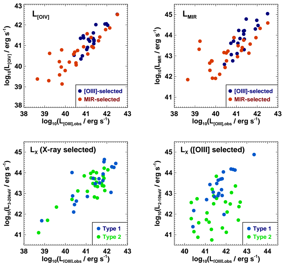
Fig. 7.— Relationships between different estimators of bolometric luminosity for radiative-mode AGN. Top panels: a comparison of the [OIII] emission line luminosity with the [OIV] line luminosity (left) and mid-infrared continuum luminosity (right), for samples of galaxies selected from their [OIII] emission line and their 12\mu\text{m} mid-IR flux (data from LaMassa et al. 2010). Bottom panels: the hard X-ray vs. [OIII] luminosity for X-ray selected (left) and emission-line selected (right) samples of AGN (data from Heckman et al. 2005). Type 2 AGN in the emission line selected samples do not show a good correlation due to X-ray absorption.
