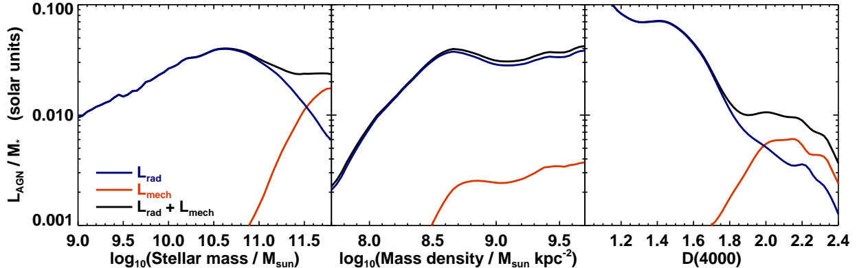
Fig. 16.— The distribution of AGN luminosity per unit stellar mass amongst galaxies from the SDSS main galaxy sample, as a function of galaxy stellar mass (left), stellar surface mass density (middle) and 4000Å break strength (right). In each plot the blue line indicates the radiative luminosity output (estimated from the [OIII] emission line), the red line shows the mechanical luminosity output in the radio jet, and the black line shows the sum of the two.
