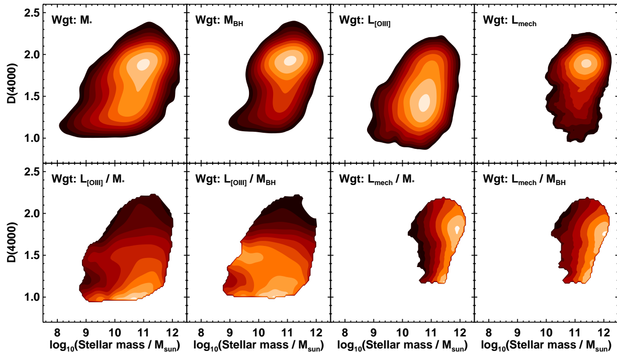
Fig. 14.— Top panels: the distribution of galaxies from the SDSS main galaxy sample in the plane of stellar mass vs. 4000Å break strength, weighted according to (from left to right): stellar mass; black hole mass; reddening-corrected [OIII] line luminosity (ie., bolometric radiative luminosity); jet mechanical luminosity. Each color band corresponds to a factor of two difference, increasing from dark to light. Bottom panels: ratios of upper panels (same color coding) to illustrate the distributions of (from left to right): bolometric radiative luminosity per stellar mass; bolometric radiative luminosity per black hole mass; jet mechanical luminosity per stellar mass; jet mechanical luminosity per black hole mass.
