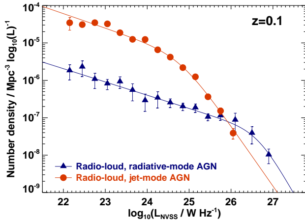
Fig. 11.— The local radio luminosity function of radio-loud AGN, split into radiative-mode and jet-mode sources. The data are largely drawn from the results of Best & Heckman (2012) who split these two populations and derived luminosity functions using radio-selected AGN in the SDSS main galaxy sample. However, as shown by Gendre et al. (2013), these results under-estimate the luminosity function of the radiative-mode AGN above 10^{26} \text{ W Hz}^{-1} , where Type-1 AGN dominate. Therefore the results of Gendre et al. are adopted for the three highest luminosity points of the radiative-mode population. The local radio luminosity functions are well-fitted by broken power law models.
