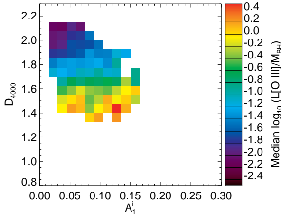
Fig. 19.— The relationship between L_{[\text{OIII}]} / M_{\text{BH}} , D4000, and galaxy lopsidedness ( A_1^i ). The color coding of these two-dimensional histograms indicates the median L_{[\text{OIII}]} / M_{\text{BH}} . The primary correlation is between stellar age and L_{[\text{OIII}]} / M_{\text{BH}} , as is apparent from the horizontal nature of the color contours. There is no independent correlation between L_{[\text{OIII}]} / M_{\text{BH}} and lopsidedness in these data. Figure from Reichard et al. (2009).
