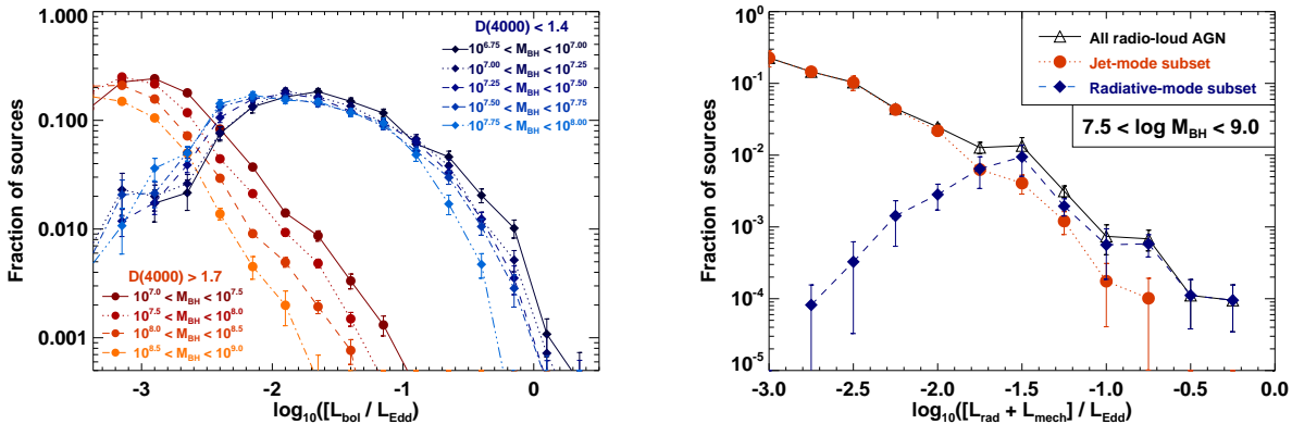
Fig. 12.— Left: the distribution of Eddington-scaled accretion ratios for emission-line selected AGN from the SDSS main galaxy sample, split by star-formation activity. Following Kauffmann & Heckman (2009), the distributions are shown separately for actively star-forming host galaxies ( D(4000) < 1.4 ) and for passive host galaxies ( D(4000) > 1.7 ), each for a range of black hole masses. Fractions plotted are within each 0.25-dex wide bin in Eddington ratio. As found by Kauffmann & Heckman, the passive galaxies show a power-law distribution of Eddington fractions, the amplitude of which decreases with increasing black hole mass. In contrast, the Eddington ratios of the star-forming hosts show a log-normal distribution peaking at a few percent of Eddington. This distribution is largely independent of black hole mass (though this depends slightly upon the version of the M - \sigma relation adopted). Right: the Eddington-scaled accretion ratios of radio-loud AGN from SDSS, split into jet-mode and radiative-mode sources; again, fractions plotted are within each 0.25-dex wide bin. Here the bolometric luminosity is calculated by summing the radiative and mechanical contributions. The two classes show distributions remarkably similar to the populations seen for emission-line AGN in the left panel.
