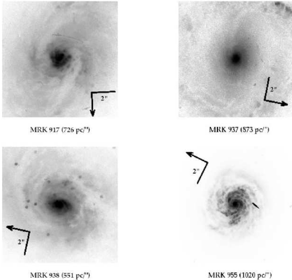
Fig. 20.— HST optical images of the central regions of four typical Type 2 Seyfert galaxies from Malkan et al. (1998). The arrowhead points North and the bar points East, and the angular scale is indicated. Note that the linear scale (pc per arcsec) quoted in each case assumed H_0 = 50 \text{ km s}^{-1} \text{ Mpc}^{-1} . In all these examples the central few-kpc-scale region shows the spiral arms and dust lanes typical of pseudo-bulges.
