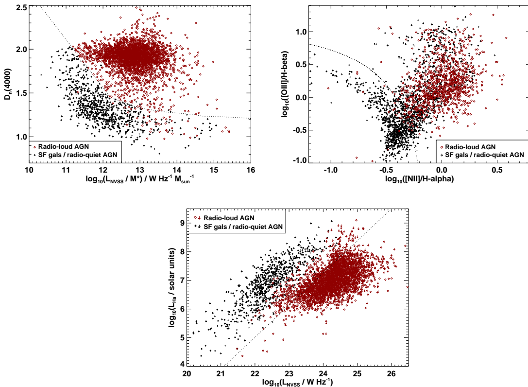
Fig. 6.— Diagnostic diagrams showing the galaxies within the SDSS main galaxy sample that are detected in the radio waveband above S_{1.4\text{GHz}} = 5 mJy. These diagrams are used to separate genuine radio-loud AGN from other radio-detected galaxies in which the radio emission is powered by star-formation (this includes both radio-quiet AGN and star-forming galaxies). The upper-left plot shows the ‘D(4000) vs. L_{1.4\text{GHz}}/M ’ method, originally developed by Best et al. (2005a). The upper-right plot shows the widely-used ‘BPT’ emission line ratio diagnostic. The lower plot shows the relationship between H\alpha and radio luminosity (arrows indicate upper limits to the H\alpha luminosity). In all plots, the dotted lines indicate the division used by Best & Heckman (2012) for that classification method. For the ‘BPT’ diagnostic diagram, this division separates AGN from star-forming galaxies in terms of what powers the emission lines, rather than what powers the radio emission. The division line in the L_{H\alpha} vs. L_{1.4\text{GHz}} plot was defined to ensure a clean sample of genuine radio-loud AGN below the division. Through combinations of the locations of galaxies in the three diagrams (see Best & Heckman for details) sources can be given an overall classification as radio-loud AGN (red diamonds) or star-forming galaxies / radio quiet AGN (black crosses). Adapted from Best & Heckman (2012).
