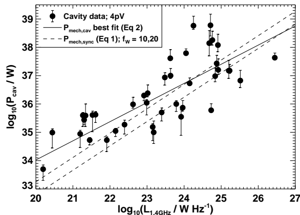
Fig. 8.— The jet mechanical energy of radio sources, estimated as 4pV from cavities and bubbles in the X-ray gas, versus the monochromatic 1.4 GHz radio luminosity. Data are primarily sourced from Cavagnolo et al. (2010), Birzan et al. (2008) and Rafferty et al. (2006). The solid line indicates the best-fit linear relation, given in Eq 2. For comparison, the dotted lines show the synchrotron estimate of Eq 1, for values of f_W = 10 and 20.
