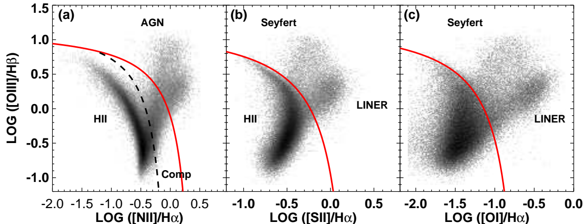
Fig. 5.— A set of BPT diagnostic diagrams for the SDSS main galaxy sample taken from Kewley et al. (2006). The red line is the maximal starburst line from Kewley et al. (2001) while the dashed line in the left panel shows the more stringent dividing line between pure star-forming galaxies and AGN adopted by Kauffmann et al. (2003a). The separation between star-forming galaxies and AGN is most cleanly done using the left panel while the center and right panels can be used to separate Seyferts from LINERs.
