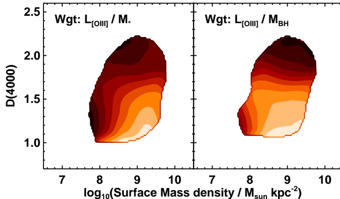
Fig. 17.— The distributions of AGN bolometric radiative luminosity per unit galaxy stellar mass (left) and bolometric radiative luminosity per black hole mass (right) in the stellar surface mass density vs. 4000Å break strength plane. [Color-banding as in Fig. 14]. Radiative-mode AGN activity clearly requires both an abundant supply of cold gas (indicated by recent or on-going star formation) and a high stellar surface mass density.
