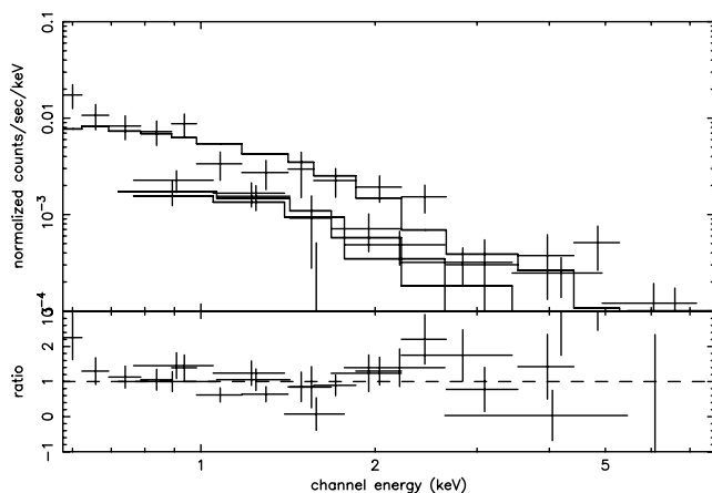
Figure 12. X-ray spectra of C11054–1145 extracted from the MOS (lower points) and pn (upper points) cameras and best-fitting thermal emission model (histograms). Residuals are shown in the lower panel.
