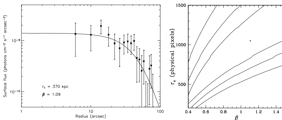
Figure 11. Left-hand panel: radial surface flux profile for C11054–1145 obtained by masking point sources and summing exposure-corrected, background-subtracted counts within annuli. Right-hand panel: corresponding constraints on \beta and r_c . The r_c axis is in XMM physical pixels which are 0.05 arcsec on a side. The contours mark 1, 2 and 3 \sigma levels.
