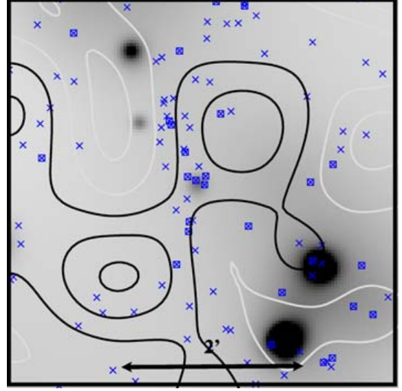
Figure 16. Adaptively smoothed 0.5–8 keV X-ray image of the central region of the C11040–1155 field with the Clowe et al. (2006) weak-lensing mass reconstruction of the field overlaid. Contour intervals are \sim 1 \times 10^8 M_{\odot} \text{ kpc}^{-2} relative to the local mean, with negative contours shown in light grey. The crosses indicate sources for which spectra have been obtained; the squares indicate spectroscopically confirmed cluster members. North is up and east is to the left-hand side.
