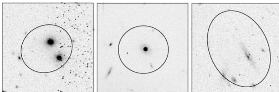
Figure 13. Candidate cluster AGN in C11054–1145. From left-hand side: C11054_X9, C11054_X10, and C11054_X26. The boxes are 15 arcsec on a side, north is up, and east is to the left-hand side. The ellipses are the 3 \sigma uncertainty of the XMM position.
