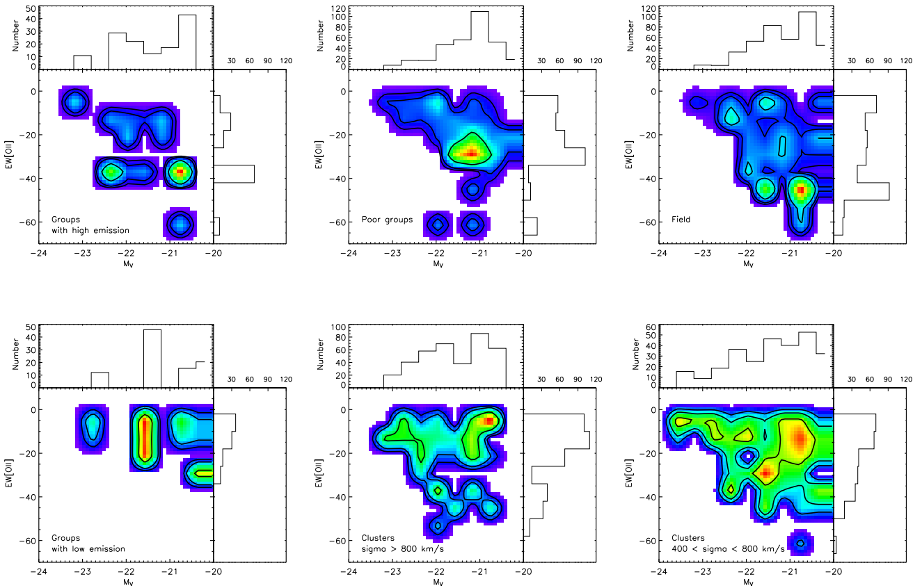
FIG. 12.— Number density maps of star-forming galaxies in different environments as a function of galaxy absolute V magnitude and EW([OII]) . Contours represent 25, 75 and 90 percentiles, while the color scale is meant to guide the eye. The histograms on top and on the right present the number of galaxies in bins of absolute magnitude and EW([OII]) , respectively. Numbers in this figure have been corrected for spectroscopic incompleteness. The raw (uncorrected) numbers of galaxies are 39 (massive clusters), 126 (less massive clusters), 31 (groups with high emission), 19 (groups with low emission), 51 (poor groups) and 75 (field).
