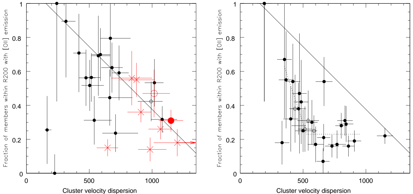
FIG. 4.— Left. The [OII] - \sigma relation in clusters at 0.4 \leq z \leq 0.8 . The fraction of cluster members within R_{200} with [OII] emission is plotted versus the cluster velocity dispersion. Solid black dots represent EDisCS datapoints in each one of the 18 fields, as in Table 1. The red solid large circle is the cluster MS1054-03 from van Dokkum et al. and the red empty circle is C11324+3011 from Postman et al. Errorbars on the fractions are Poissonian. The solid line across the plot is taken as a description of the upper envelope of the high- z points (see text). The same line is repeated in the right panel, to illustrate the differences. At high- z , the majority of systems group around this line, while at low- z (right panel) the great majority fall well below the line. Right. The [OII] - \sigma relation in low redshift clusters from Sloan described in §4. Empty circles indicate those Sloan clusters slightly outside of the preferred redshift range. The two dotted lines represent the eye-fitted most heavily populated region in the plot.
