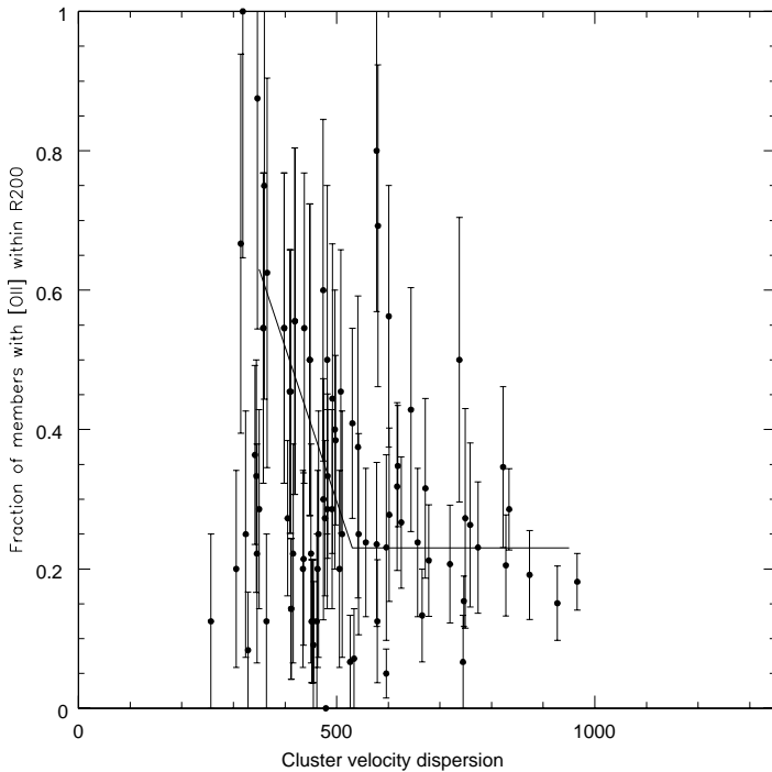
FIG. 6.— The [OII] - \sigma relation in Sloan clusters at 0.04 < z < 0.08 taken from the C4 catalog (Miller et al. 2005). Errorbars on the \sigma have been omitted for clarity. The two lines indicate the trend followed by the Abell sample, as the dotted lines in the right panel of Fig. 4.
