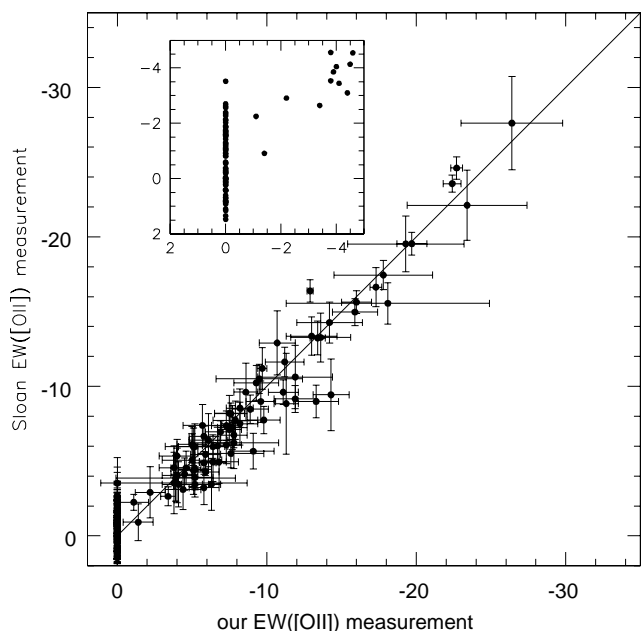
FIG. 3.— EW([OII])s of Sloan spectra in plate #973. The measurement obtained with the Ediscs method is compared with the EW listed by Sloan. The inset is a blow-up of the lower left corner of the plot, in which errorbars are omitted for clarity. In this plot, EDisCS EWs = 0 correspond to those spectra in which the line is not detected and the spectral fluctuations in that region are considered noise. Since the Sloan measurements are fully automatic, these cases can yield a non-null negative or positive EW value, that is however consistent with zero within the errorbar in most cases.
