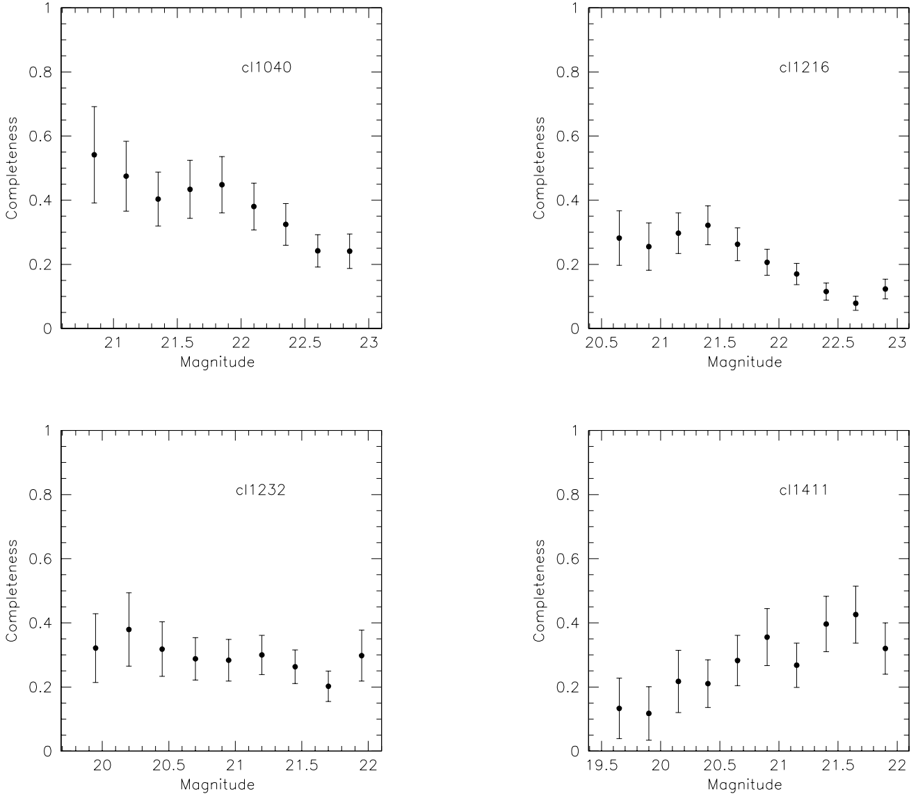
FIG. 17.— Completeness functions versus galaxy magnitudes for four EDisCS clusters.
