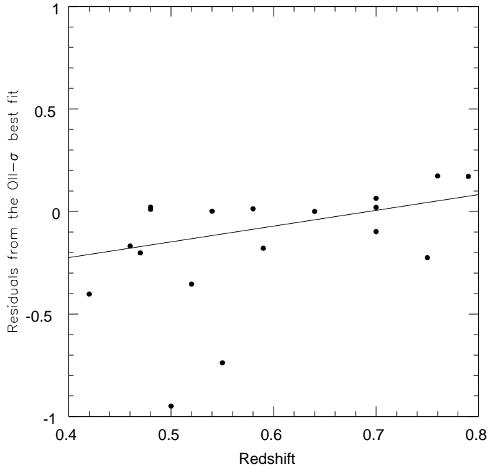
FIG. 5.— Residuals of the [OII] fraction of EDisCS clusters with respect to the line drawn in the [OII] - \sigma relation at high- z shown in Fig. 4, plotted versus cluster redshift. The solid line is the least squares fit having excluded the two outliers (Cl 1119 and Cl 1420), which are the two points with residuals < -0.5 .
