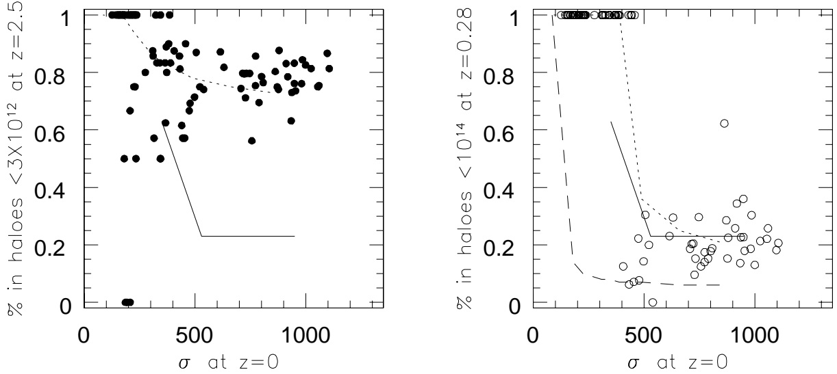
FIG. 16.— Clusters at low redshift. Comparison between the [\text{OII}] - \sigma relation observed at low redshift (solid broken line) and results from the Millennium Simulation (dots) and from the Press-Schechter formalism (dotted lines). Left. The solid broken line traces the [\text{OII}] - \sigma relation observed at low redshift. Dots represent the fraction of galaxies in 90 haloes in the MS simulation that were in haloes with mass < 3 \times 10^{12} at z=2.5 . The dotted line is the prediction of the fraction of mass in haloes < 3 \times 10^{12} at z=2.5 for a system of a given \sigma at z=0.0 derived from the Press-Schechter formalism. Right. The solid broken line is repeated from the left panel. Empty dots represent the fraction of galaxies in 90 haloes from the MS simulation that were in haloes with mass < 10^{14} \sim 3 Gyr prior to observations, thus at z=0.28 . The short dashed line is the prediction of the fraction of mass in haloes < 10^{14} at z=0.28 for a system of a given \sigma at z=0.0 derived from the Press-Schechter formalism. The long dashed line is the prediction of the fraction of mass in haloes < 3 \times 10^{12} at z=0.28 for a system of a given \sigma at z=0.0 derived from the Press-Schechter formalism.
