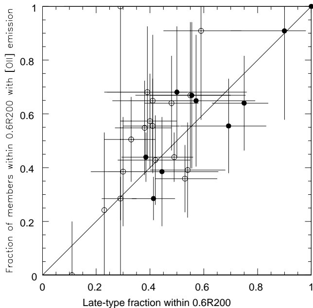
FIG. 13.— [OII] fraction of EDisCS clusters versus the fraction of late-type galaxies, both computed within 0.6R_{200} and down to M_V = -20.0 . The late-type fraction is computed as the fraction of spectroscopically confirmed members. Empty dots represent the fraction of late-type galaxies obtained from structural parameters derived from 2D bulge+disk decompositions of VLT images (Simard et al., 2006). Filled dots represent the fraction of late-type galaxies (all galaxies excluded ellipticals and S0s) derived from visual morphological classifications of HST images (Desai et al., 2006). The 1:1 line is shown for comparison.
