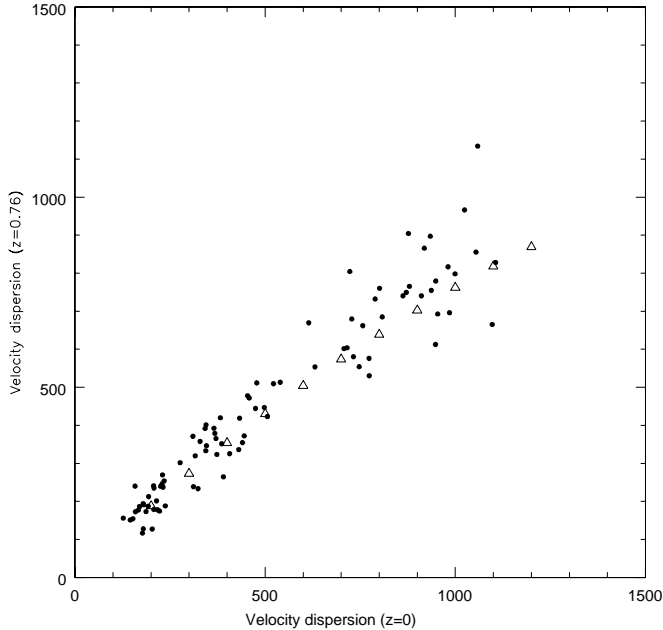
FIG. 8.— Relation between the velocity dispersion of systems at z=0 and at z=0.76 . Empty triangles are average values derived analytically from Wechsler et al. (2002) and eqn.4, as described in §5.2. Filled circles are results for 90 haloes from the Millennium Run simulation (Springel et al. 2005), as described in §5.2.
