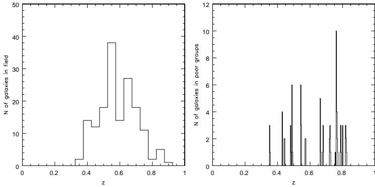
FIG. 9.— Left. Redshift distribution of our field spectroscopic sample. Right. Redshift distribution of galaxies in our poor groups.
