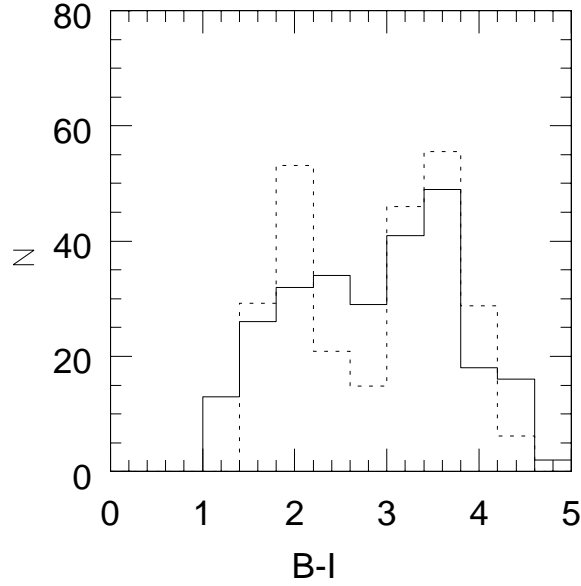
FIG. 18.— Color distributions of the parent photometric catalog (solid line) and of the spectroscopic catalog corrected for incompleteness (dashed line) for the cluster C 1202.
