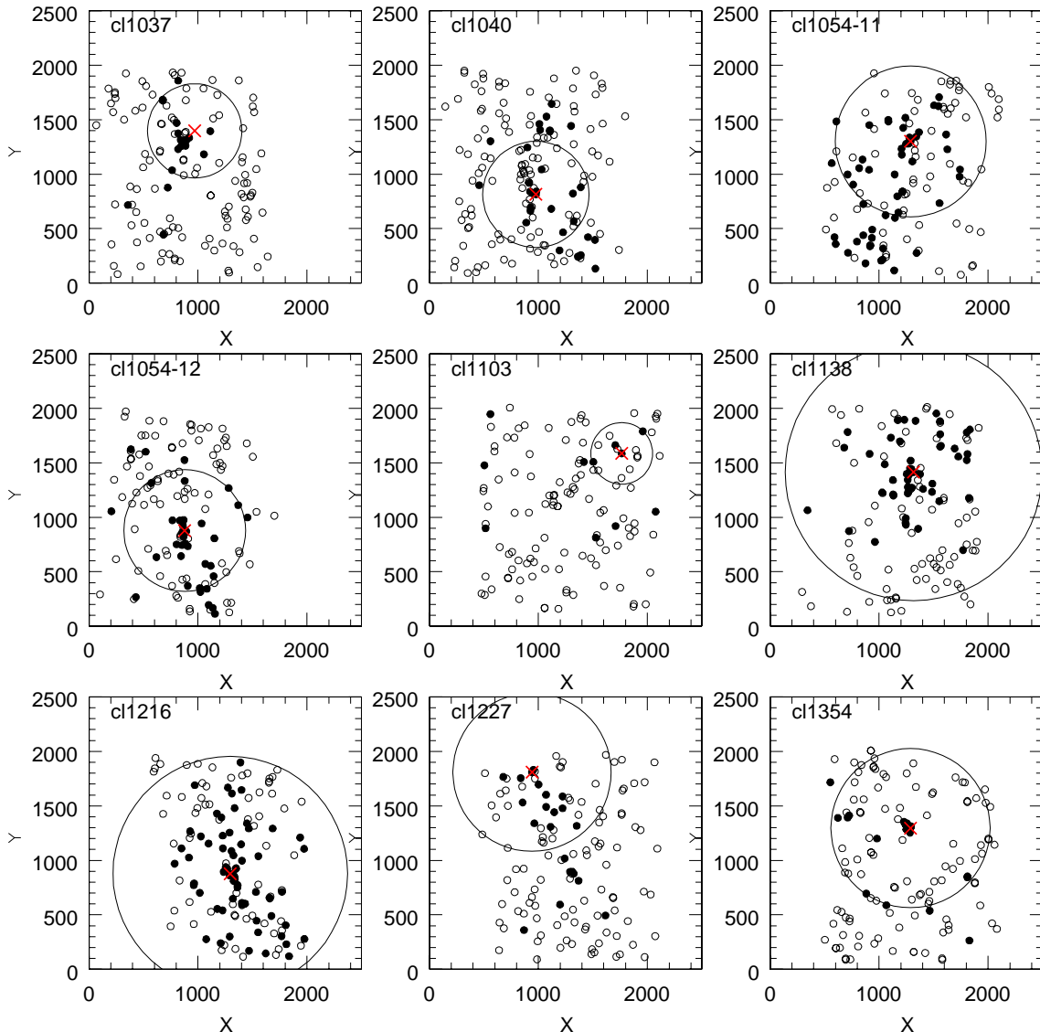
FIG. 2.— Same as Fig. 1 but for the high- z EDisCS fields.
