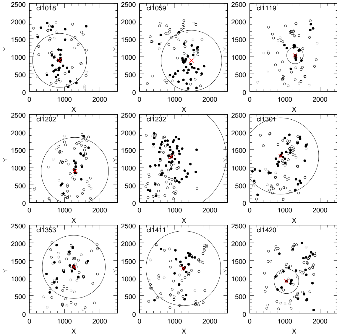
FIG. 1.— XY pixel positions of objects with spectra in the EDisCS mid- z fields. Filled dots represent spectroscopically confirmed cluster members. The circle with radius R_{200} , centered on the BCG, is shown. The axis units are pixels = 0.2'' .
