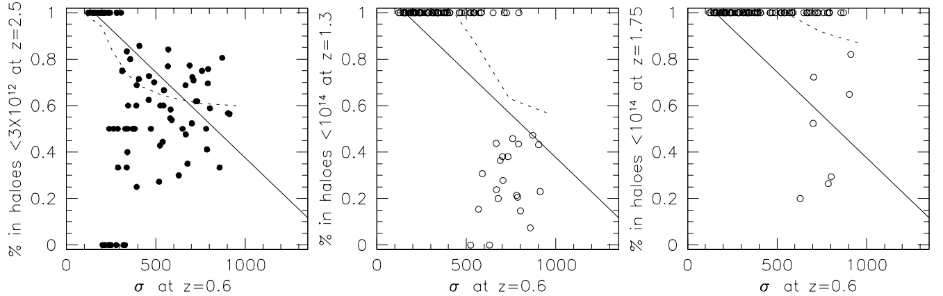
FIG. 15.— Clusters at high redshift. The solid line is the line drawn in the [OII] – \sigma diagram observed at high redshift. Left. Dots represent the fraction of galaxies in 90 haloes selected at z=0.6 in the MS simulation that were in haloes with mass < 3 \times 10^{12} at z=2.5 . The dotted line is the prediction of the average fraction of mass in haloes < 3 \times 10^{12} at z=2.5 derived from the Press-Schechter formalism. Middle. Empty dots represent the fraction of galaxies in the MS simulation that were in haloes with mass < 10^{14} \sim 3 Gyr prior to z=0.6 , thus at z=1.3 . The dotted line is the prediction of the fraction of mass in haloes < 10^{14} at z=1.3 derived from the PS. Right. Empty dots represent the fraction of galaxies in the MS simulation that were in haloes with mass < 10^{14} \sim 3 Gyr prior to z=0.8 , thus at z=1.75 . The dotted line is the prediction of the fraction of mass in haloes < 10^{14} at z=1.75 derived from the PS.
