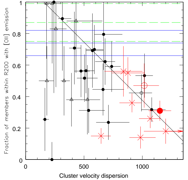
FIG. 10.— Same as Fig. 4, but now including also other environments. Empty triangles are other EDISCS structures with at least 7 spectroscopically confirmed members as in Table 5. The average [OII] fraction and corresponding errorbars in poor groups (those between 3 and 6 spectroscopic members) are shown with green dashed lines. The [OII] fraction among field galaxies (see text) and its errorbars are shown as blue solid lines.
