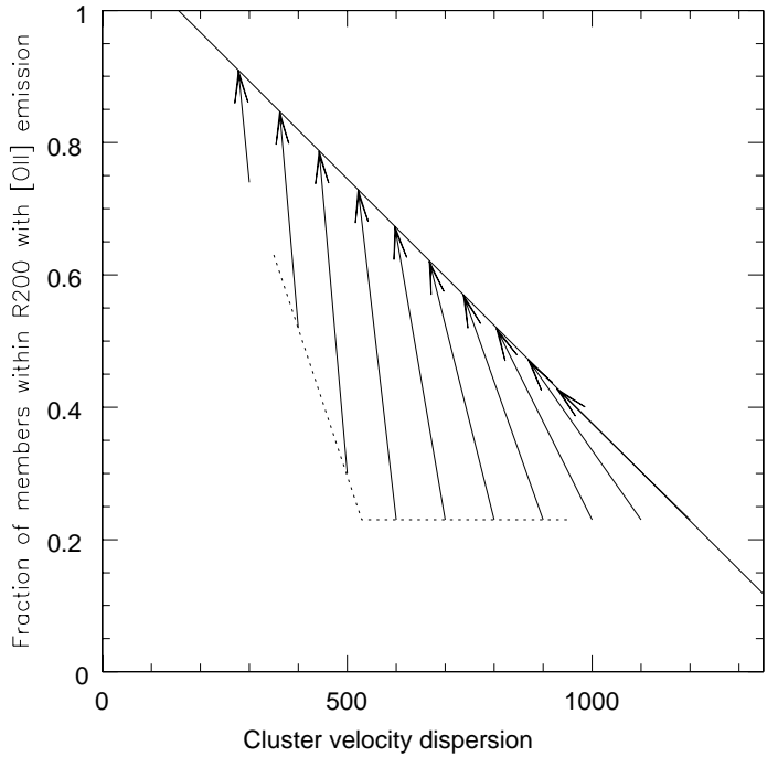
FIG. 7.— Evolution of the [OII] - \sigma relation inferred from observations at different redshifts. The solid line and the two dotted lines represent the observed relations followed by the majority of clusters at high- and low- z , respectively. These are the same lines shown in the left and right panels of Fig. 4. The arrows identify the average progenitors at z = 0 of clusters of different mass at z = 0 as expected from simulations, considering the fact that the cluster mass, hence its velocity dispersion, evolves too (see text for details). If \sigma did not evolve with time, the arrows would be vertical in this plot.
