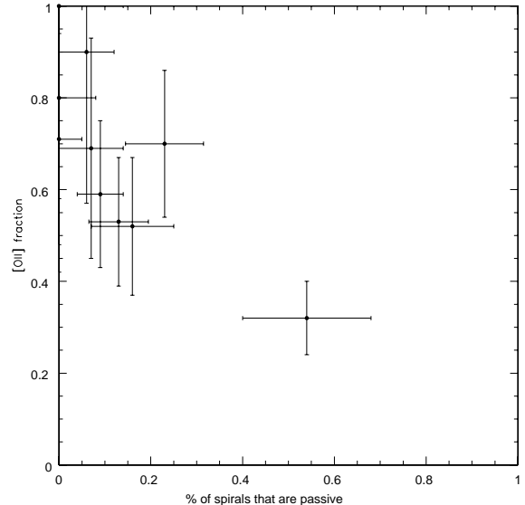
FIG. 14.— Fraction of late-type galaxies (spirals+irregulars from HST images) that are passive (lack emission lines in their spectra) versus [OII] fraction for EDisCS systems.
