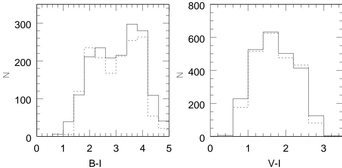
FIG. 19.— Left. Color distribution of the parent photometric catalog (solid line) and the spectroscopic catalog corrected for completeness (dashed line) for the 9 clusters with B photometry. Right. As left panel, for clusters with V photometry.
