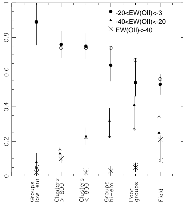
FIG. 11.— Fraction of star-forming galaxies with a strong, moderate and relatively weak equivalent width of [OII] in different environments. Environments are located on the x-axis in order of increasing average [OII] fraction as from Fig. 4. The fraction of galaxies with relatively low EW ( -20 < EW < -3 \text{ \AA} , circles) decreases going to environments with higher [OII] fraction. The fraction of galaxies with intermediate-strength EW (triangles) follows the opposite trend. The fraction of galaxies with strong EW (crosses, EW < -40 \text{ \AA} ) is higher in the field than in any other environment, and a possible excess is observed in massive clusters compared to the other environments. Filled symbols and solid line crosses refer to values corrected for incompleteness, while the uncorrected values are shown as empty symbols and dotted crosses.
