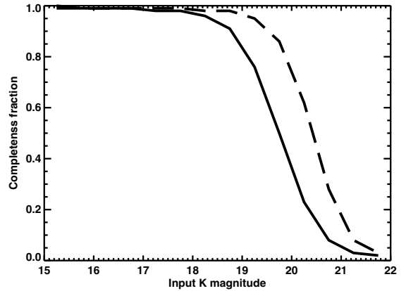
Figure 1. The completeness fraction for both stellar (dashed line) and galactic (solid line) model objects as a function of input magnitude, averaged over all 28 fields.
