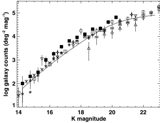
Figure 6. The K -band galaxy number counts per magnitude per square degree, in \Delta K = 0.5 mag intervals. The solid symbols represent the data presented in this paper and tabulated in Table 1; for K < 19 the values plotted are those from ‘all fields’ and for K > 19 they are those from the five deep fields only. The other symbols represent data from the literature: open squares and (point-up) triangles are, respectively, the bright and faint samples of Minezaki et al. (1998); diamonds are from Djorgovski et al. (1995); circles are from Moustakas et al. (1997); crosses are from Szokoly et al. (1998); asterisks, inverted triangles and stars are, respectively, the Hawaii Medium Deep Survey, the Hawaii Deep Survey and the Hawaii Medium Wide Survey presented by Gardner et al. (1993); open crosses are from McLeod et al. (1995); bow-ties ( \bowtie ) are from Bershadsky et al. (1998). The solid line represents a passive luminosity evolution model, discussed in Section 4.3.
