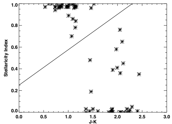
Figure 4. A plot of stellaricity index against J - K colour: stars generally have bluer colours and higher stellaricity indices than galaxies, and so combining these two parameters allows fairly accurate star–galaxy separation. The stars lie to the upper left of the line. The field plotted here is 3C22, chosen for this demonstration because of its high fraction of stars.
