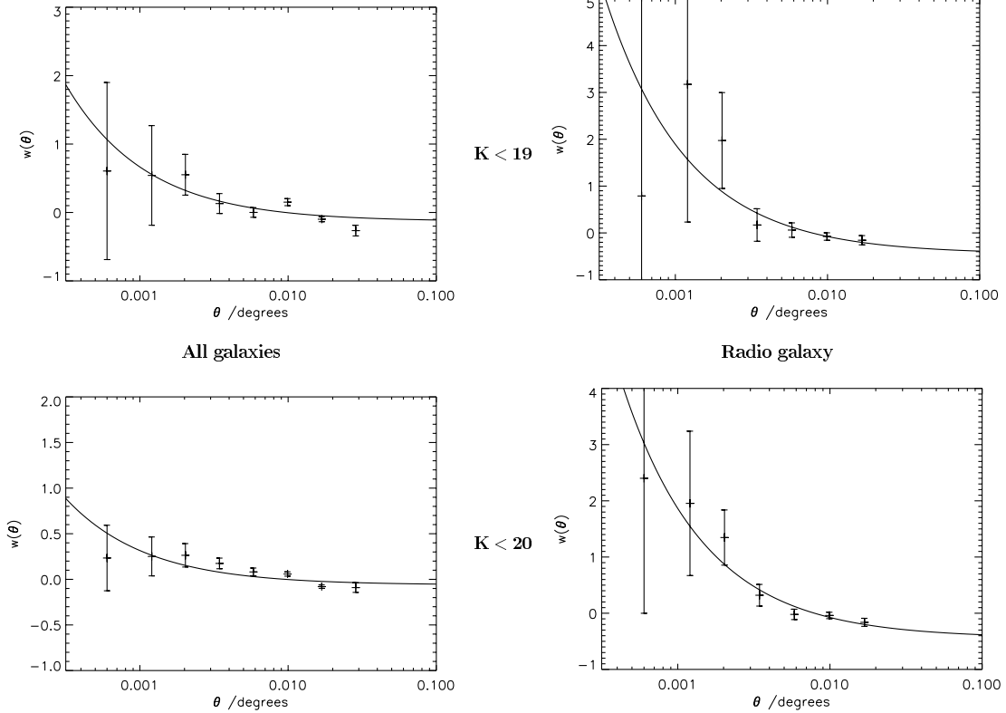
Figure 7. The angular cross-correlation function for all galaxy–galaxy pairs (left) and for just the radio galaxy–galaxy pairs (right) averaged over all of the UKIRT K -band images. The upper plots include all galaxies with K < 19 , to which level the observations are almost complete; the lower plots include galaxies down to K < 20 , at which level there is a significant completeness correction, but the number statistics are increased. The plots are fit with functions of the form w(\theta) = A\theta^{-0.8} - C , where C is the integral constraint and has a value of C_{\text{gg}} = 41.1A_{\text{gg}} for all galaxy–galaxy pairs, and C_{\text{rg}} = 48.0A_{\text{rg}} for just radio galaxy–galaxy pairs (see text).
