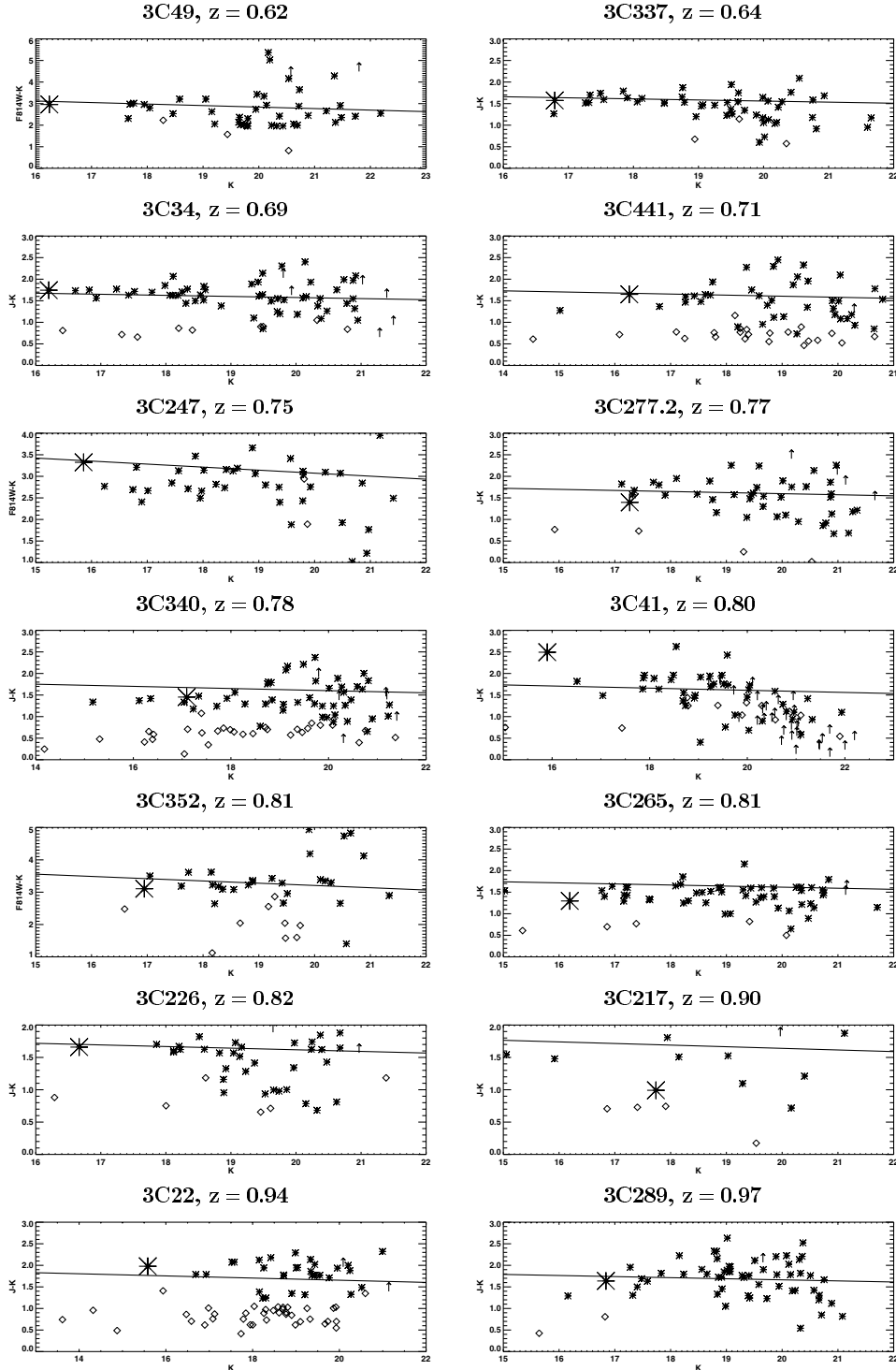
Figure 8. Near-infrared colour–magnitude relations for the 3CR radio galaxies. The fields and redshifts are labelled above each diagram. Galaxies are represented by asterisks and stars by open diamonds. Upper limits are plotted as an arrow for a galaxy and as an arrow plus a diamond symbol for a star. The large plotted symbol represents the radio galaxy. The solid lines display the colour–magnitude relations that would be obtained by simply passively evolving the colour–magnitude relation observed in the Coma cluster back in redshift, assuming an elliptical galaxy which formed its stars in a short time-span at z = 10 .
