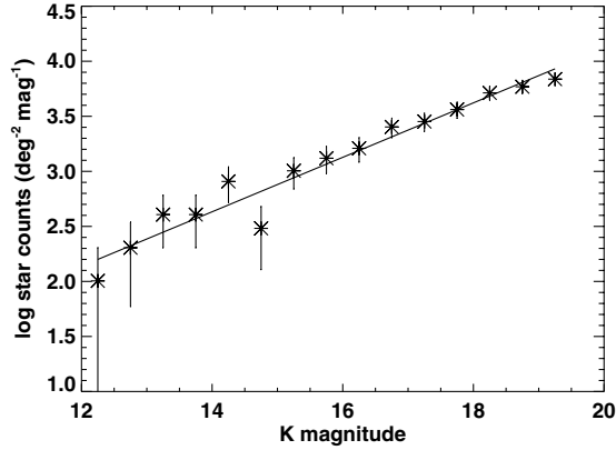
Figure 5. The differential star number counts in the K -band, in \Delta K = 0.5 mag intervals, fit using a single power-law distribution.
