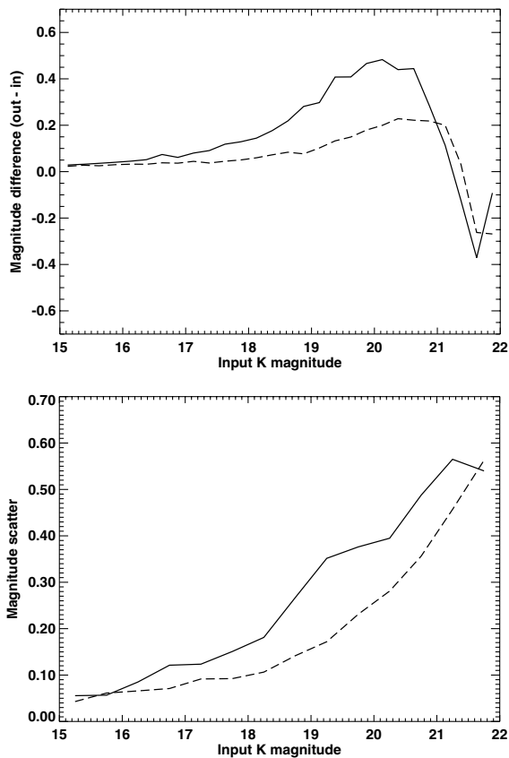
Figure 3. The mean (upper plot) and rms scatter (lower plot) of the difference between the measured magnitudes and the input magnitudes for the model stars (dashed line) and galaxies (solid line).
