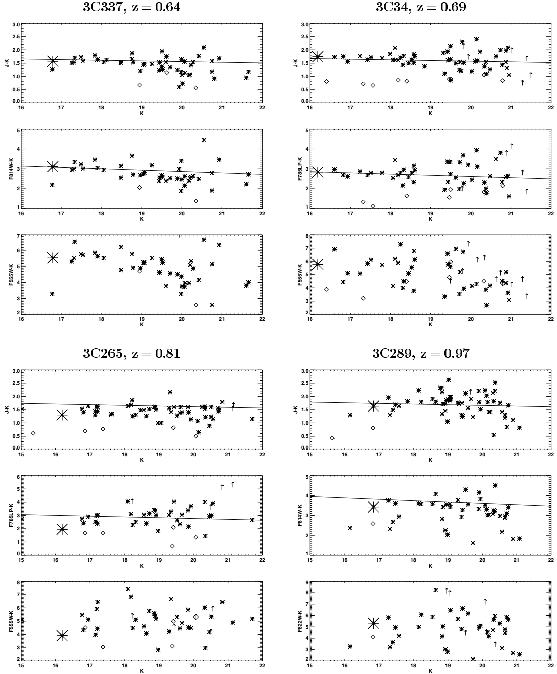
Figure 9. Colour–magnitude relations for the 3CR radio galaxies from the UKIRT and HST data. Symbols as in Fig. 8. The redshifted Coma colour–magnitude relations are only plotted on figures for which both filters are to the long-wavelength side of the rest-frame 4000 Å break, since below that wavelength small quantities of recent or on-going star formation can have large effects on the colours leading to only poorly defined sequences.
