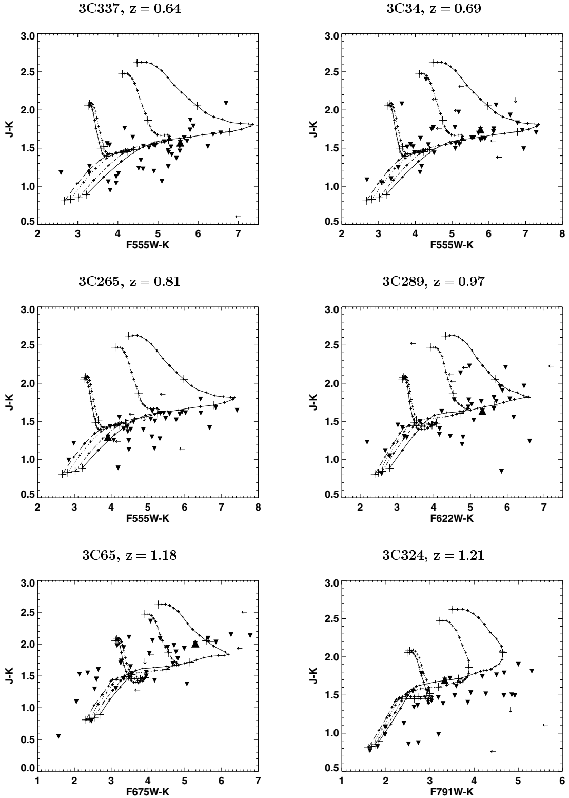
Figure 10. Colour–colour plots for fields of the six radio galaxies presented in Fig. 9. The large triangle represents the radio galaxy, and the smaller upside-down triangles represent the other galaxies in the field. Galaxies with upper limits on their colours are indicated by arrows. The four tracks show the colour evolution of the passively evolving galaxy models described in Section 4.3: Es, solid line; Sabs, dot-dash line; Scs, dotted line; Sdms, long-dashed line. The tracks run from z = 0 (lower left of plot) to z = 3 , with the small crosses along each line representing steps of 0.1 in redshift, and redshifts z = 0, 1, 2, 3 being indicated by the larger crosses.
