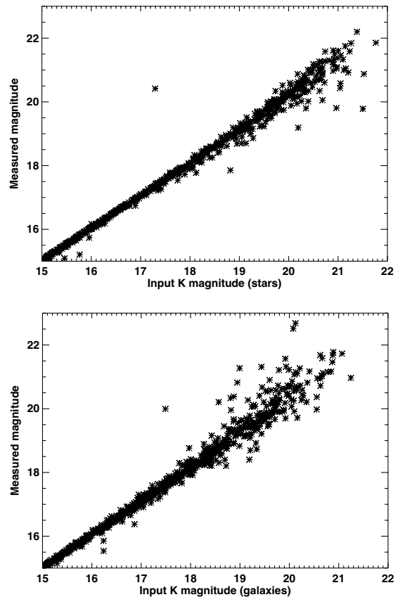
Figure 2. The distribution of measured magnitudes as a function of input magnitudes for the model stars (upper plot) and galaxies (lower plot). The plots are for 1000 model objects. No point is plotted if the model object is not detected by SEXTRACTOR.
