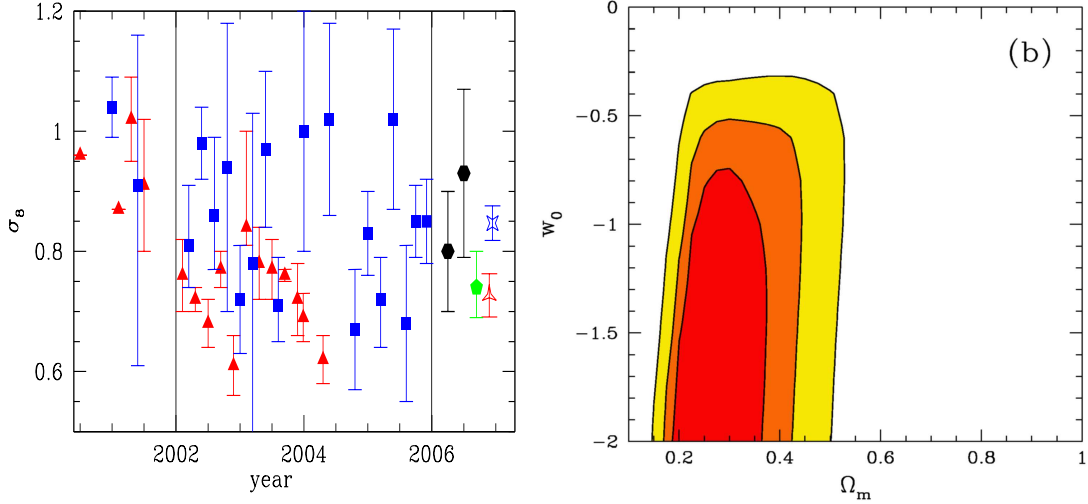
Figure 17: Left: a compilation of the most recent determination of \sigma_8 from the analysis of clusters of galaxies (red) and cosmological weak lensing. From Hettterscheidt et al. (2006). Right: constraints on dark energy derived from the CFHTLS Deep and Wide weak lensing survey, assuming a constant w and a flat universe. From Hoekstra et al. (2006).
