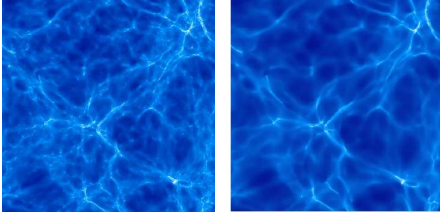
Figure 25: Numerical simulations of the matter distribution of a cold/warm (left/right) dark matter model. The reduced small scale structure due to the free-streaming of the warm dark matter ( m_{\text{WDM}} = 0.5 \text{ keV} ) is clearly seen and well probed by the Ly \alpha forest. Simulations were run with the numerical hydrodynamical code Gadget-II on the COSMOS computer in Cambridge (box-size 30h^{-1} \text{ Mpc} ).
