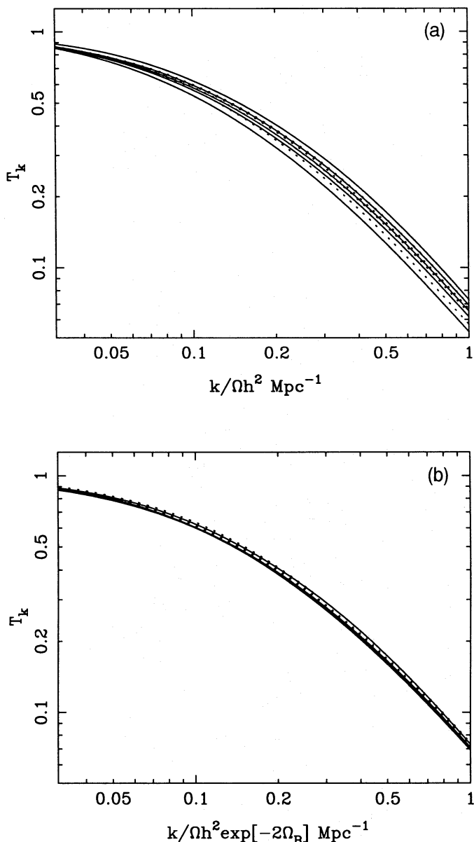
Figure 8. A set of CDM transfer functions, using the fitting formulae of BBKS for zero baryon content, and those of Holtzman (1989) for \Omega_b = 0.01, 0.03, 0.05, 0.1 . Models with h = 1 are shown as solid lines, h = 0.5 are dotted. When plotted (panel a) against k/\Omega h^2 , the varying baryon content causes variations in the curves, with higher \Omega_b producing greater suppression of power. However, this can be scaled away (panel b) by plotting against the combination k/[\Omega h^2 \exp(-2\Omega_b)] . In these terms, the CDM transfer function has a universal shape, which can be described by the zero-baryon formula of BBKS. The scaling becomes noticeably imperfect for \Omega_b \gtrsim 0.3 , but is very good for the models plotted here.
