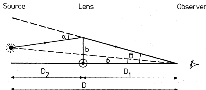
Figure 1. The geometry for a lensing event. The deflection angle \alpha is a function of impact parameter b . \theta and \phi are the angles between the lens and respectively the image and the object. The distances D , D_1 and D_2 are in general the angular-diameter distances of cosmology.
