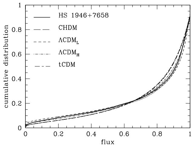
Figure 9. Comparison between the measured flux distribution of HS 1946+7658 and the model predictions. A continuum offset correction is applied to each model to enforce matching the cumulative distributions at flux values near unity. The dotted curve shows the measured cumulative flux distribution after removing pixels contaminated by identified metal lines. The best matches are obtained by the \Lambda CDM L and \Lambda CDM H models, with predicted distributions that bracket the measured one.
