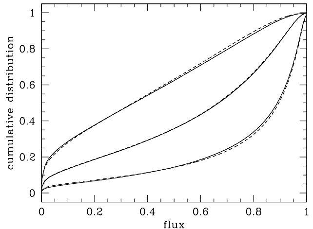
Figure A1. Test of the interpolation method for the flux distribution, for the \Lambda CDM H model. The left pair of curves show the flux distribution at z = 4 (solid curve) and the predicted distribution based on rescaling the model spectra at z = 3 according to equation (1) (dashed curve). The right pair of curves show the flux distribution at z = 3 (solid curve) and the predicted distribution from rescaling the spectra at z = 4 (dashed curve). The central pair show the flux distribution at z = 3.6 (solid curve) and the linearly interpolated distribution based on rescaling the spectra at z = 3 and z = 4 and using equation (2) (dashed curve). The predicted and actual distributions at z = 3.6 agree to within 1 per cent.
