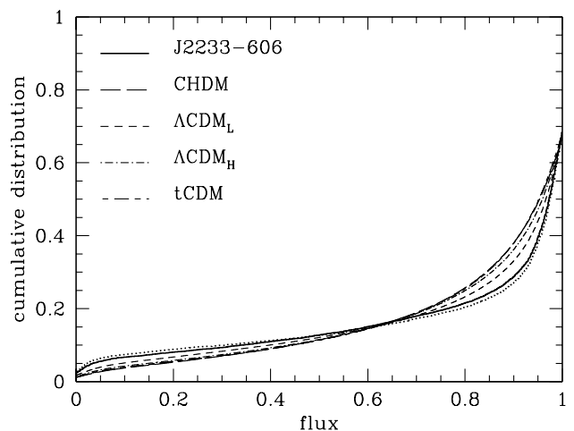
Figure 17. Comparison between the measured flux per pixel distribution of J2233–606 and the model predictions. A continuum offset was applied to each model to enforce matching the cumulative distributions at flux values near unity. None of the models recover the measured flux distribution, although the \Lambda\text{CDM}_L model is closest. The dotted line shows the measured flux distribution after removing regions contaminated by identified metal lines.
