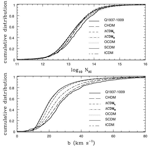
Figure 6. Comparison between the measured absorption line parameter cumulative distributions of Q1937–1009 and the model predictions using AUTOVP, allowing for an offset in the continuum level. The CHDM model agrees best with the measured N_{\text{HI}} and b distributions.
