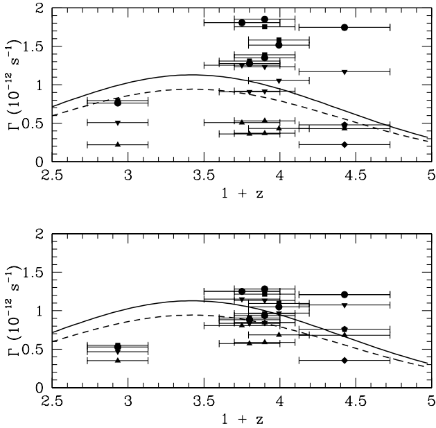
Figure 20. Required H I photoionization rate \Gamma required for the models to match the measured mean optical depths, for CHDM (circles), \Lambda CDM L (triangles), \Lambda CDM H (inverted triangles), tCDM (squares), OCDM (diamonds) and SCDM (pentagons). The upper panel shows \Gamma for the value of \Omega_b assumed in the model. The lower panel shows \Gamma assuming a fixed value of \Omega_b h^2 = 0.020 for all the models. The predicted values are close to the estimated \Gamma from QSO sources alone for an intrinsic QSO spectral index of \alpha_Q = 1.5 (solid curve) and \alpha_Q = 1.8 (dashed curve).
