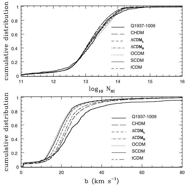
Figure 8. Comparison between the measured absorption line parameter cumulative distributions of Q1937–1009 and the model predictions using SPECFIT, allowing for an offset in the continuum level.
