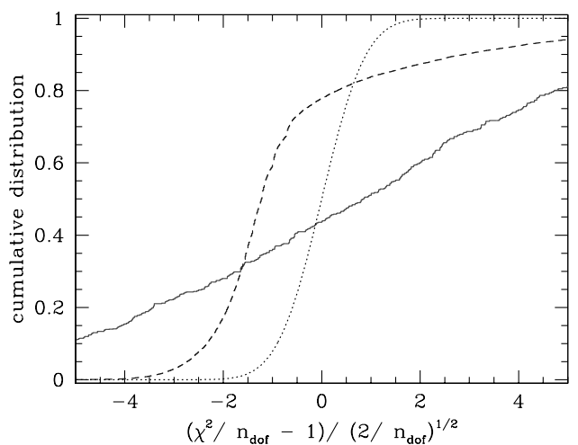
Figure A2. Distribution of \chi^2 for the absorption line fits using AUTOVP (solid curve) and SPECFIT (dashed curve), for \Lambda CDM L . Shown are the cumulative distributions of (\chi^2/n_{\text{dof}} - 1)/(2/n_{\text{dof}})^{1/2} , where n_{\text{dof}} is the number of degrees of freedom of the fit. This quantity should be distributed like a Gaussian with vanishing mean and unit variance in the limit n_{\text{dof}} \rightarrow \infty (dotted curve). Although most of the fits are acceptable, both methods produce too great a tail at large \chi^2 values.
