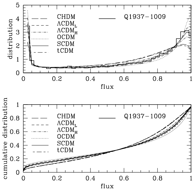
Figure 3. Comparison between the measured flux distribution of Q1937–1009 and the model predictions. A continuum offset is applied to each model to enforce matching the cumulative distributions at flux values near unity. The distributions tighten compared with Fig. 2. The SCDM model is now preferred over \Lambda CDM L . (The measured distribution has been rebinned in the upper panel for clarity.)
