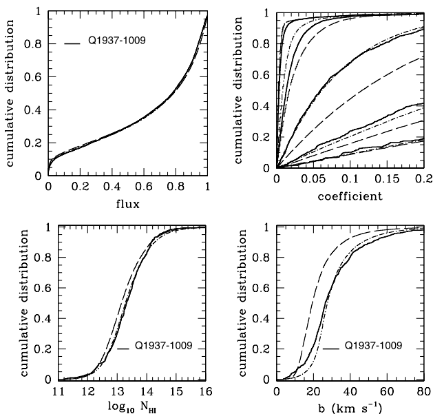
Figure 21. The effect of additional heat input owing to late HeII reionization on the predictions of the \Lambda CDM L model for Q1937–1009. Shown are the cumulative distributions of the flux per pixel (top left panel), wavelet coefficients (top right panel; labelled as in Fig. 4), H I column density (bottom left panel) and Doppler parameter (bottom right panel). The effect of late reionization is mimicked by broadening the simulation optical depths by an additional 12 \text{ km s}^{-1} (dot-dashed lines), corresponding to the expected increase in temperature owing to the onset of sudden HeII reionization. The original results without the added broadening are also shown (dashed curves), as well as the direct measurements from the spectrum of Q1937–1009 (solid curves). The extra broadening has very little effect on the flux per pixel distribution, but pronounced effects on the wavelet coefficients and fit absorption line parameters.
