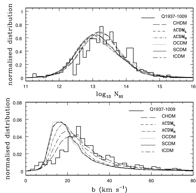
Figure 5. Comparison between the measured absorption line parameter distributions of Q1937–1009 and the model predictions using AUTOVP, allowing for an offset in the continuum level. While good agreement is generally found for the N_{\text{H I}} distributions, the predicted b distributions are generally skewed toward lower b values than measured. (The measured distributions have been rebinned for clarity of presentation.)
