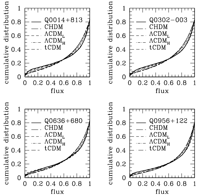
Figure 13. Comparison between the measured flux distributions of the Hu et al. (1995) QSO spectra and the model predictions. A continuum offset was applied to each model to enforce matching the predicted and measured cumulative distributions at flux values near unity. For all spectra except Q0956+122, the \Lambda\text{CDM}_L model provides the best match. For Q0956+122 the best match is given by the \Lambda\text{CDM}_H model.
