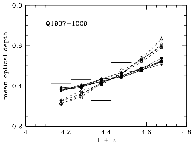
Figure 1. Redshift dependence of mean optical depth \bar{\tau}_\alpha for Q1937–1009 (horizontal bars). The open symbols show the values for \bar{\tau}_\alpha found in the simulations based on the evolution of the UV radiation background as determined from QSO sources by Haardt & Madau (1996). The filled symbols show the values for \bar{\tau}_\alpha after allowing for an alternative redshift dependence of the UV radiation background. The symbols are: CHDM (circles), \Lambda CDM L (squares), \Lambda CDM H (diamonds), OCDM (triangles), SCDM (inverted triangles) and tCDM (pentagons).
