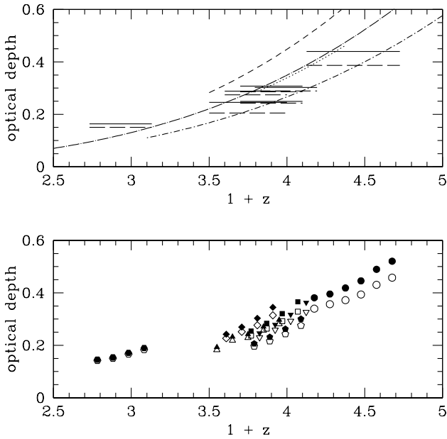
Figure 22. (Upper panel) Comparison between the total mean optical depth \bar{\tau}_\alpha (solid bars) and the effective optical depth \tau_{\text{eff}} (long dashed bars) owing to line blanketing by the Ly \alpha forest measured in the QSO spectra in Table 2. (The width of a bar indicates the redshift interval over which the optical depth is averaged.) Also shown are estimates for \bar{\tau}_\alpha using data from Steidel & Sargent (1987b) (dotted line) and Zuo & Lu (1993) (dot-dashed line), the estimate of Press et al. (1993) (short-dashed line) and the estimate of Kim et al. (2001) (dot-long dashed line). (Lower panel) The predictions of the \Lambda CDM L model for \bar{\tau}_\alpha (solid symbols) and \tau_{\text{eff}} (open symbols) for the spectra. The points near z = 3 have been slightly offset in redshift for clarity. The symbols correspond to Q1937–1009 (circles), HS 1946+7658 (triangles), Q0014+813 (inverted triangles), Q0302–003 (squares), Q0636+680 (diamonds), Q0956+122 (pentagons) and J2233–606 (hexagons).
