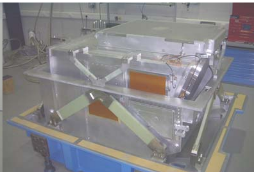
Photo 13: Trial integration of 4K stage via small truss assy.
