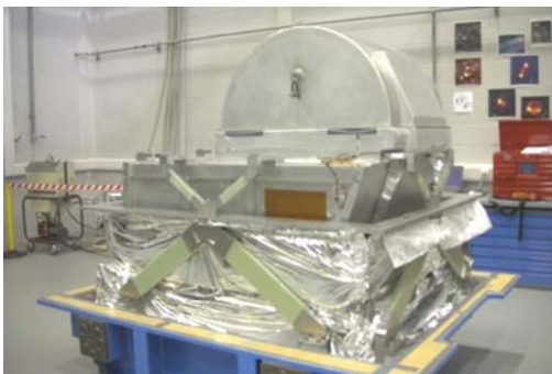
Photo 15: Real integration underway with MLI blanket.
