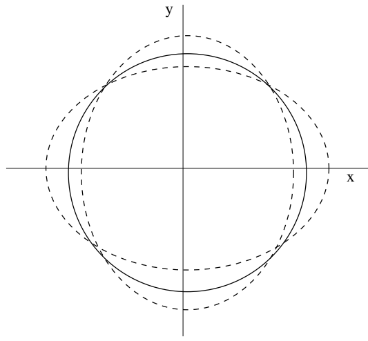
Figure 8: Effect of gravitational wave with + polarisation.
