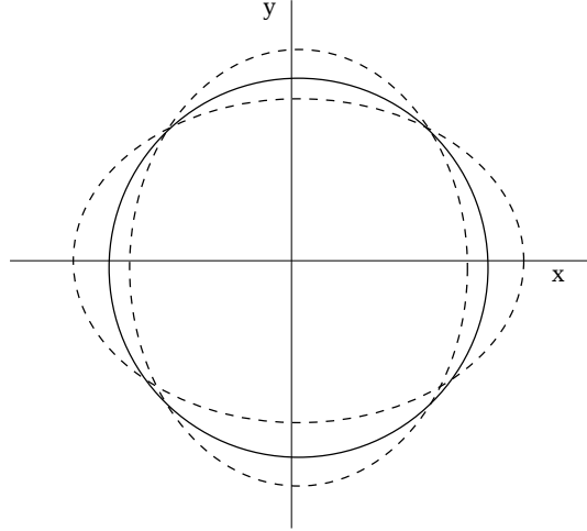
Figure 8: Effect of gravitational wave with + polarisation.
