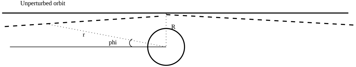
Figure 3: Light bending round the Sun.
