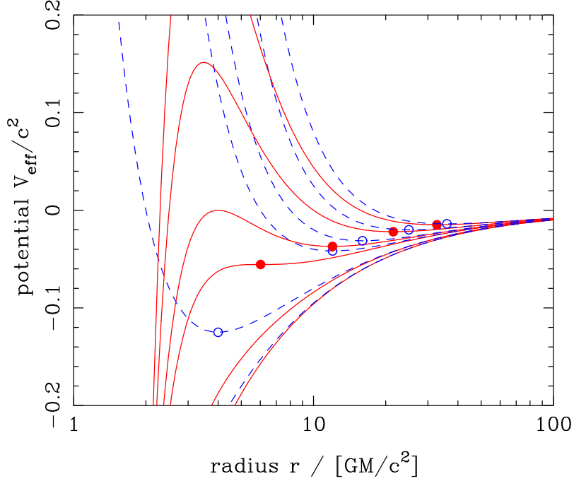
Figure 2: The effective GR potential around a point mass, and its Newtonian counterpart (dashed lines). These are plotted for different values of the dimensionless angular momentum, H = r^2 \dot{\phi} c / GM . From bottom to top, the lines are H = 1, 2, \sqrt{12}, 4, 5, 6 . Circular orbits live at minima in V_{\text{eff}} , and are plotted as points (open for Newtonian). For H < \sqrt{12} , V_{\text{eff}} has no minimum, and so there is an innermost stable orbit, at r = 6GM/c^2 .
